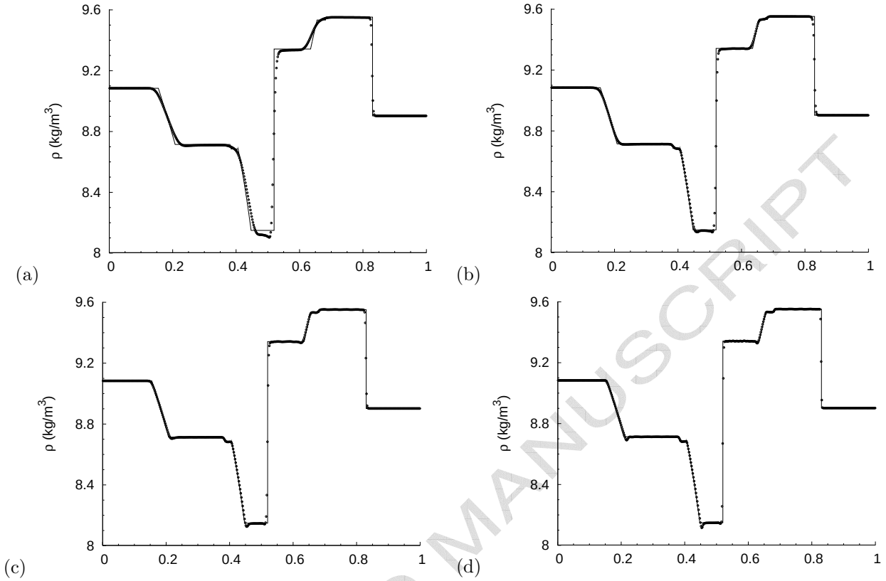
Figure 3: Comparison of exact (solid line) and numerical (points) solutions of Testcase 1 at a time t = 0.6 \mu s . Numerical solutions were obtained with a grid spacing \Delta x = 1/500 ; (a) first-order space and time with CFL=0.9; (b) WENO-3, (c) MPWENO-5, (d) MPWENO-9, all with CFL=0.6.
