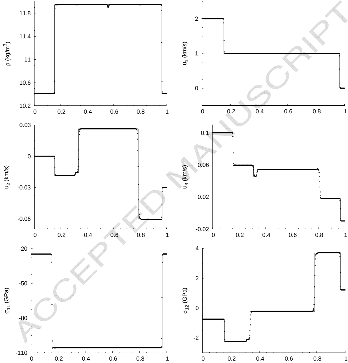
Figure 4: Comparison of exact (solid line) and numerical (points) solutions of Testcase 2 at time t = 0.6 \mu s . Numerical solutions were obtained with a grid spacing \Delta x = 1/500 , CFL=0.6, and using the 5th order WENO reconstruction scheme.
