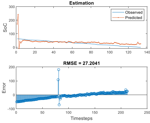
Figure 11. Initial SoC 60%
