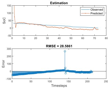
Figure 12. Initial SoC 30%
