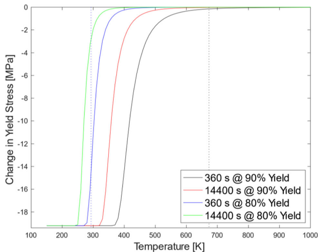
Fig. 13—Predicted softening after cycling at 80 pct or 905 of the yield stress and waiting for 360 and 14400 s. Room temperature is enough to erase softening history within minutes when cycling at 80 pct of the yield stress, but not for 90 pct of the yield stress.
