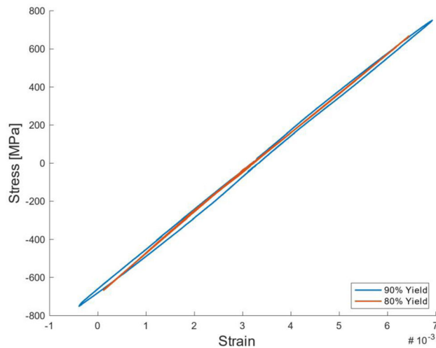
Figure A1—Stress-strain loop for 80 and 90 pct of yield stress loading at 293 K.
