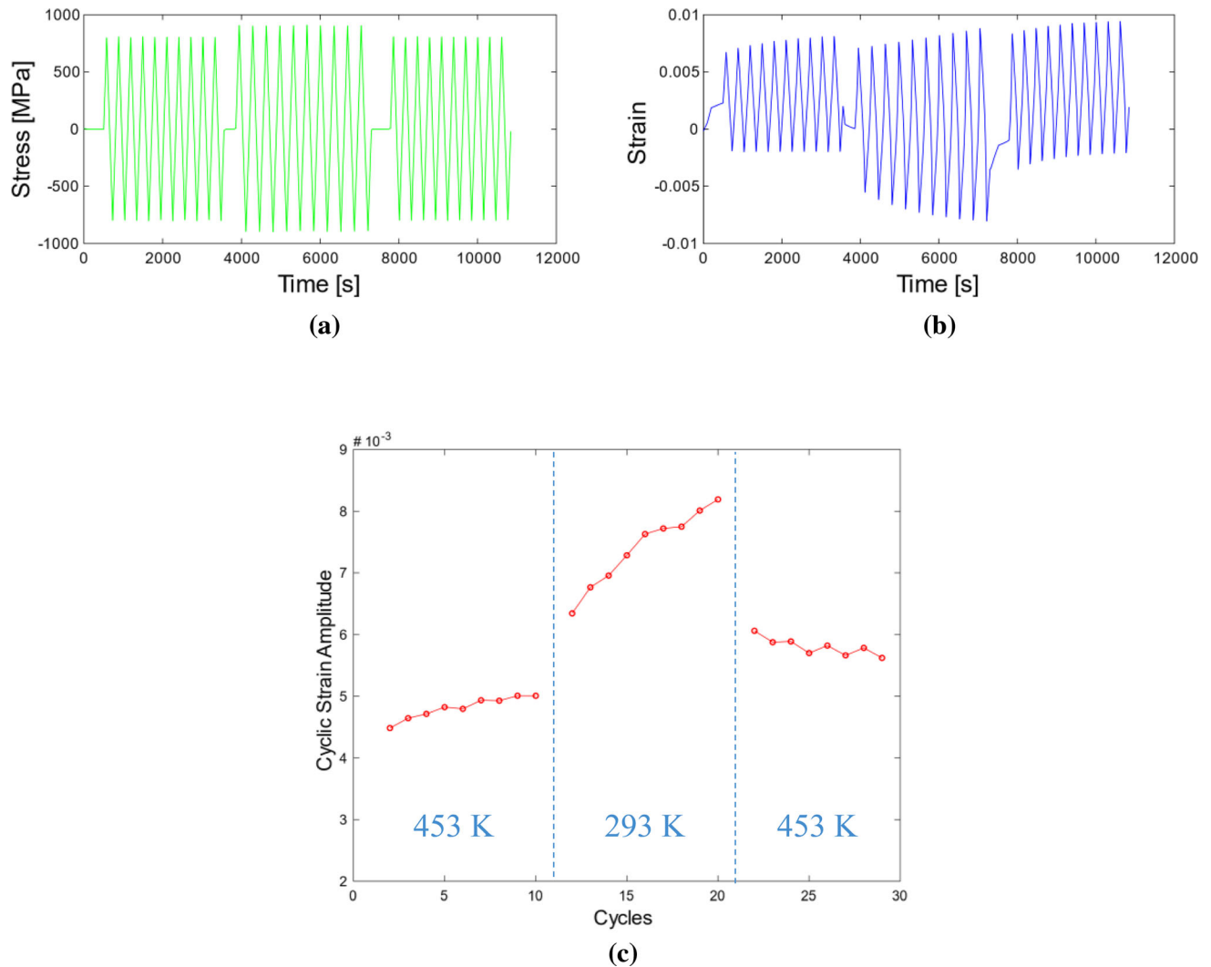
Fig. 6—Stress (a) and strain (b) responses as a function of time under constant stress amplitude of 90 pct of yield stress starting at 453 K for 10 cycles, followed by 10 cycles at 293 K, and ending with 10 cycles at 453 K. Temperature transitions occurs within 360 s (6 min). (c) Evolution of the cyclic strain amplitude in which some pronounced softening is evident during cycling at room temperature.
