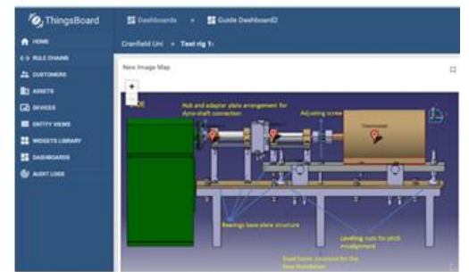
Fig. 4: The physical gearbox transmission test rig for emulating misalignment cases
