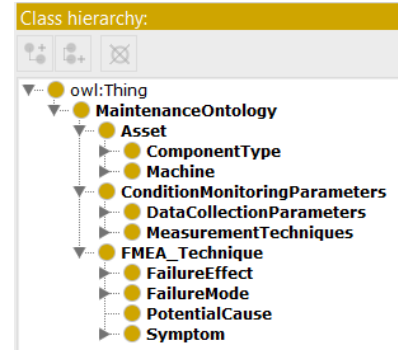
Fig. 2: Ontology classes
