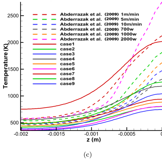
Figure 13. Temperature distribution with different laser power and welding speeds in comparison with the results of Abderrazak et al. [13] along x , y and z lines
