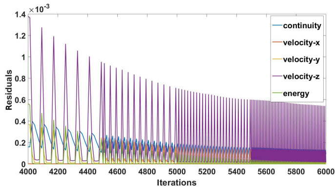
Figure 6. Residuals with CFL = 1 at 120 ms on the coarse mesh
