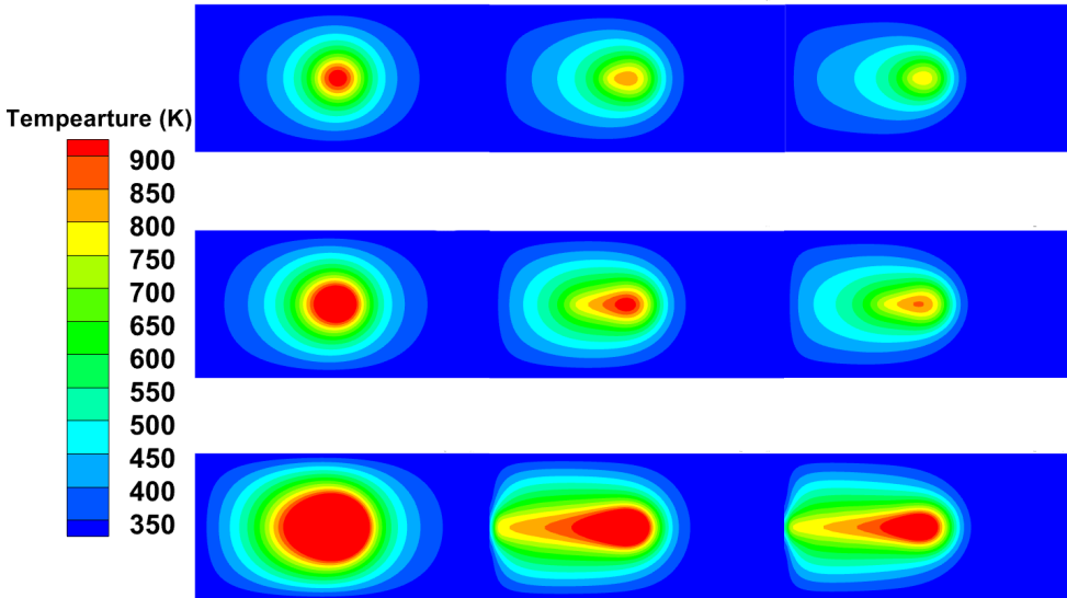
Figure 10. Temperature distribution with different parameters on x - y plane
