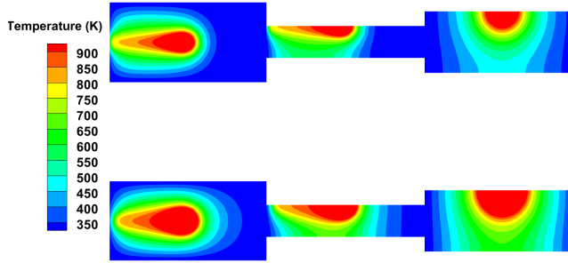
Figure 25. Temperature with and without taking the convective term into account
