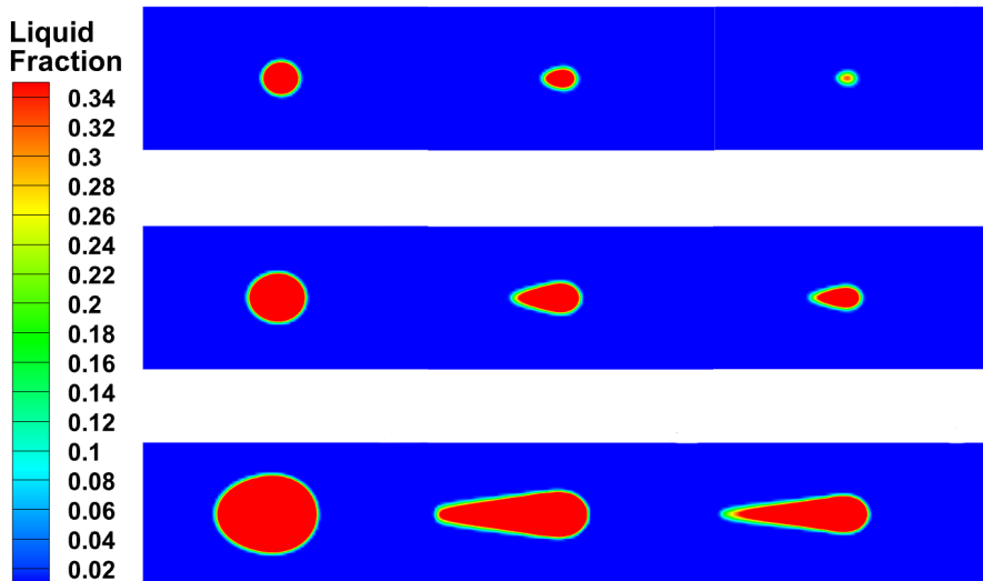
Figure 17. Liquid fraction with different parameters on x - y plane
