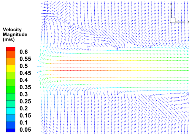
Figure 31. Velocity vector for Case 10
