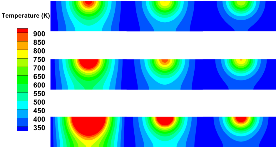
Figure 12. Temperature distribution with different parameters on y - z plane
