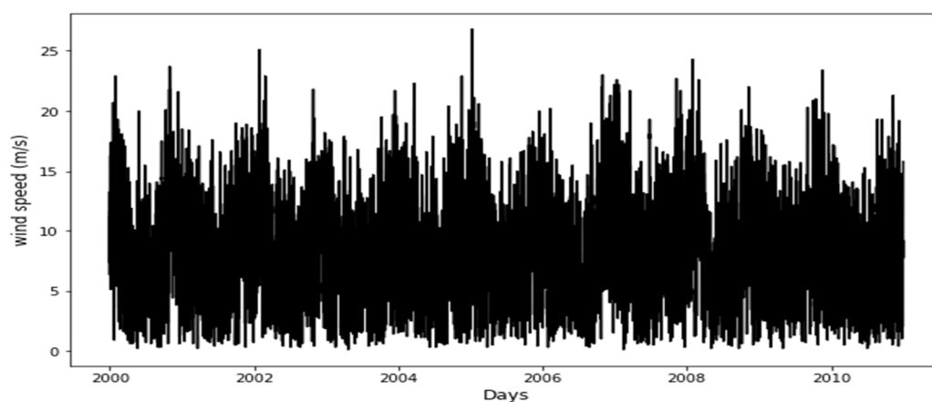
Figure 3. Raw measured wind speed datasets.
