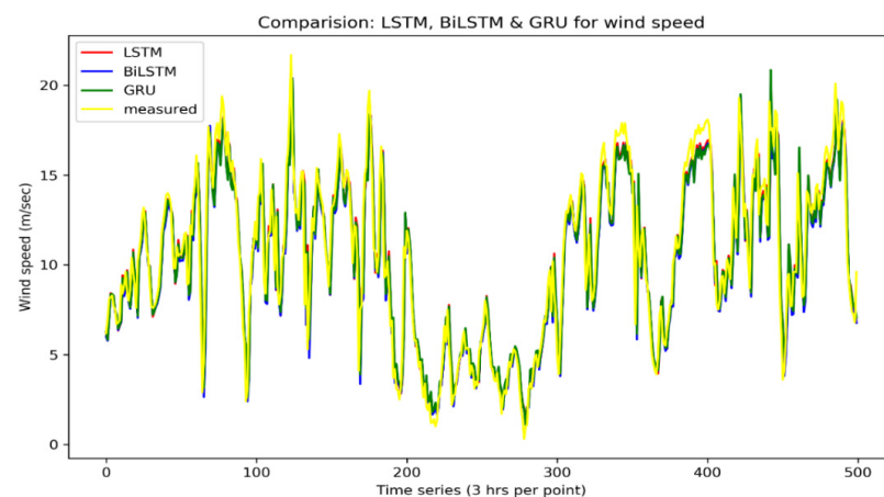
Figure 23. Performance comparison: wind speed.
