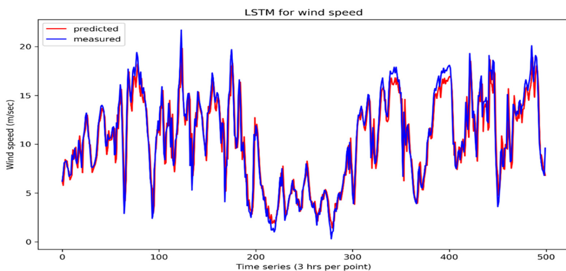
Figure 9. LSTM wind speed prediction.
