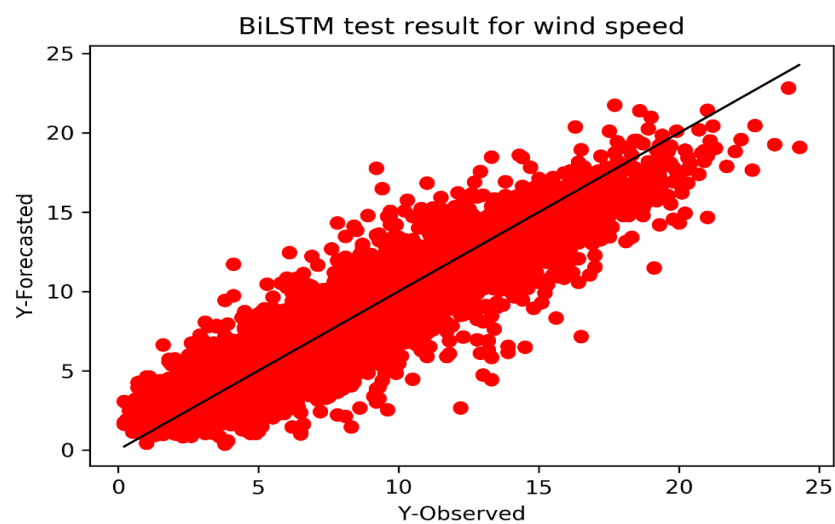
Figure 16. BiLSTM-based wind speed model error analysis.
