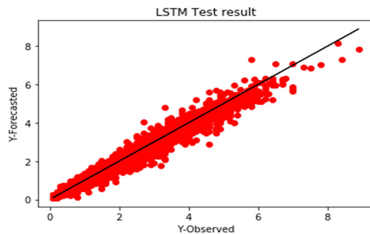
Figure 12. LSTM-based wave height model error analysis.
