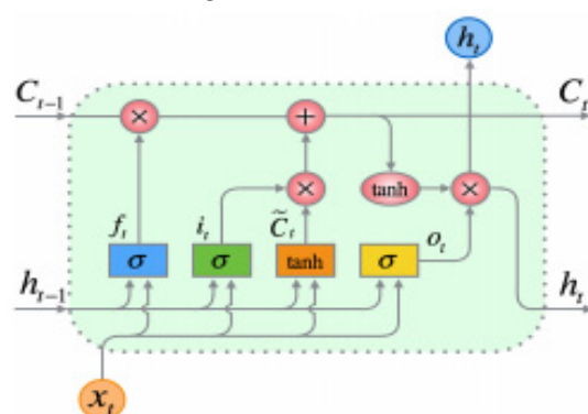
Figure 8. Overview of LSTM architecture [40].
