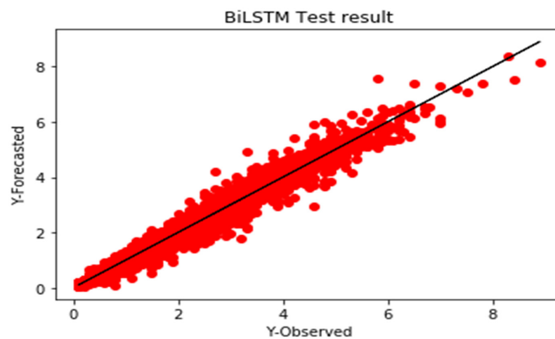
Figure 17. BiLSTM-based wave height model error analysis.
