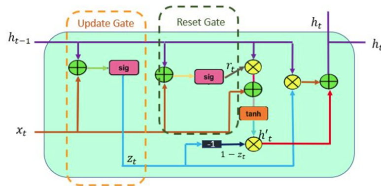
Figure 18. GRU structure overview, [43].
