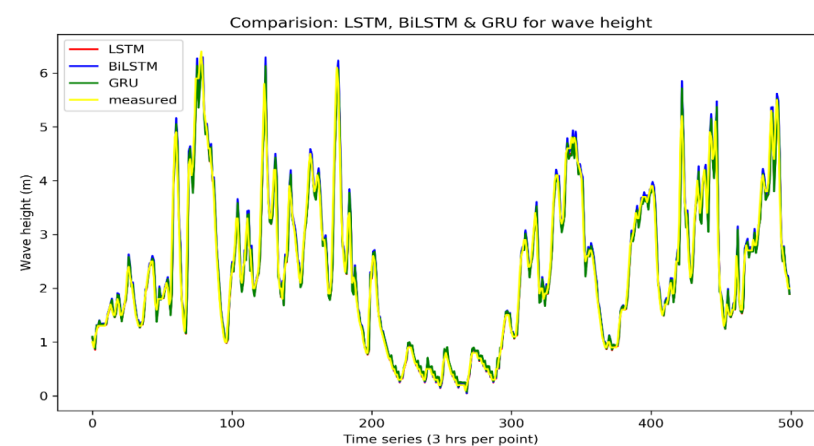
Figure 24. Performance comparison: wave height.
