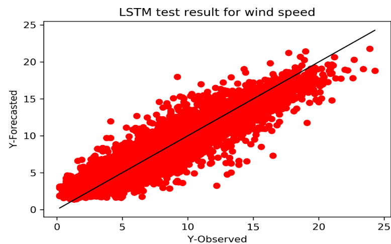
Figure 11. LSTM-based wind speed model error analysis.
