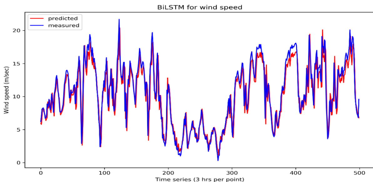
Figure 14. BiLSTM wind speed prediction.
