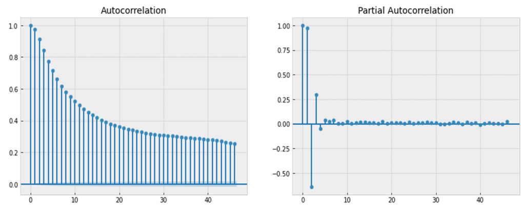
Figure 6. Wave height autocorrelation and partial autocorrelation.
