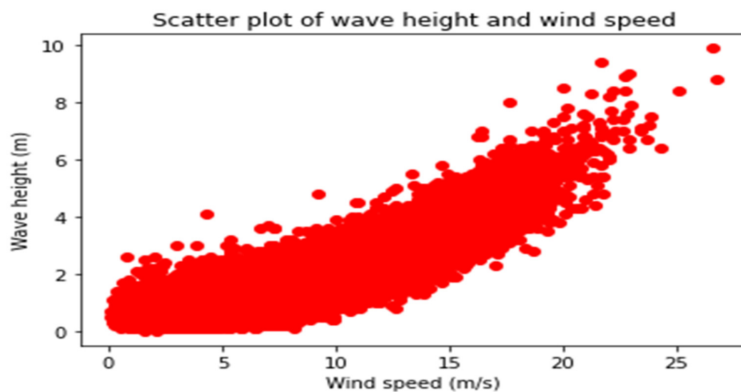
Figure 5. Scatter plot between wave height and wind speed.
