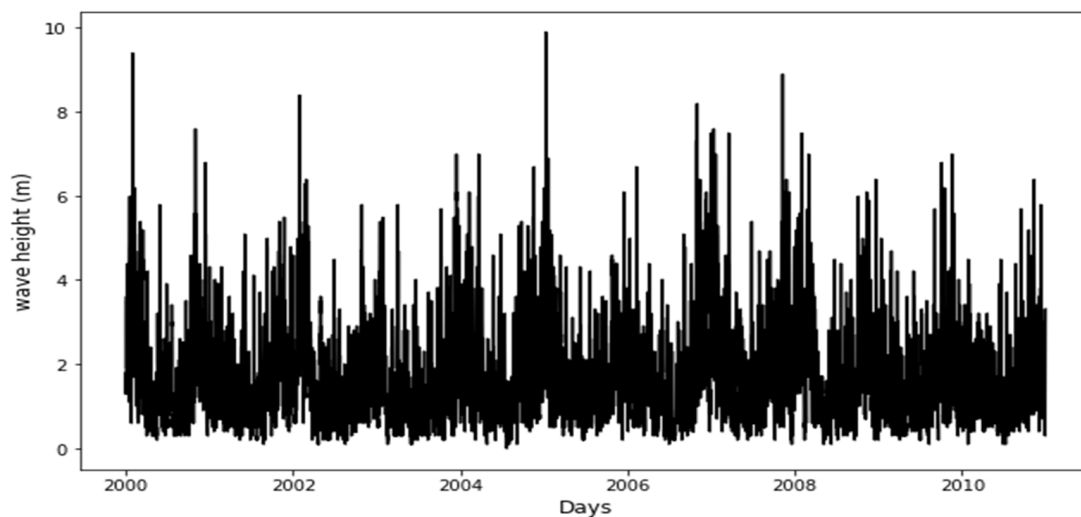
Figure 4. Raw measured wave height.
