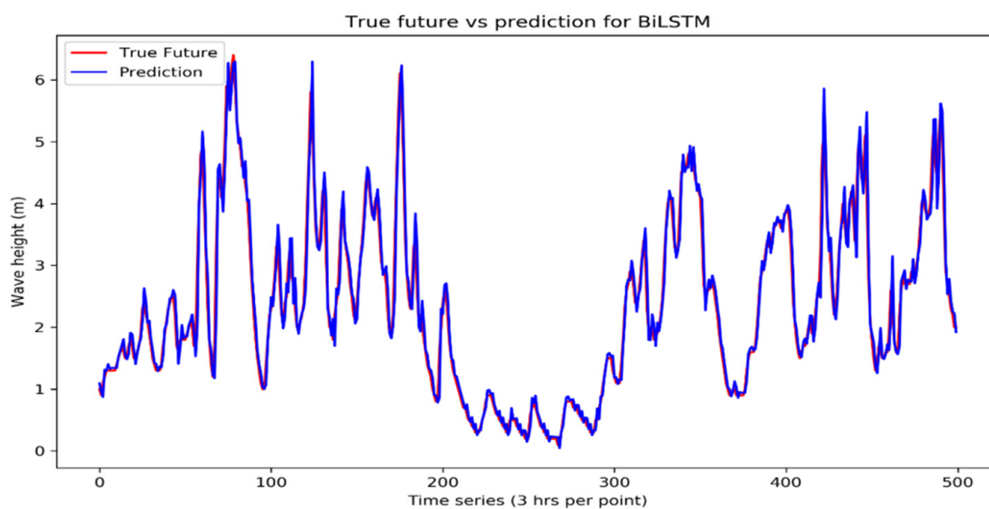
Figure 15. BiLSTM wave height prediction.
