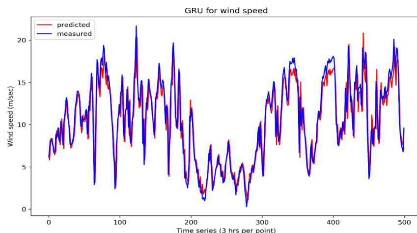
Figure 19. GRU wind speed prediction.
