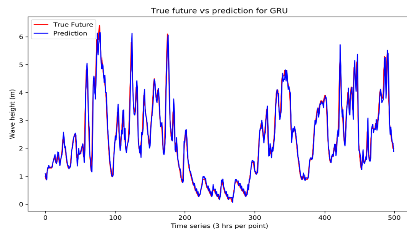
Figure 20. GRU wave height prediction.
