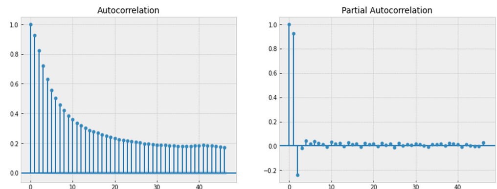
Figure 7. Wind speed autocorrelation and partial autocorrelation.
