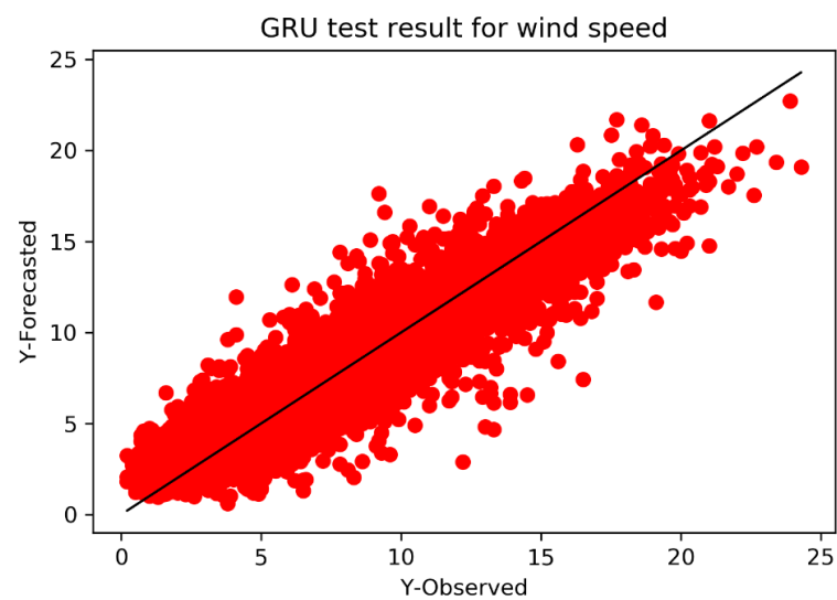
Figure 21. GRU-based wind speed models error analysis.
