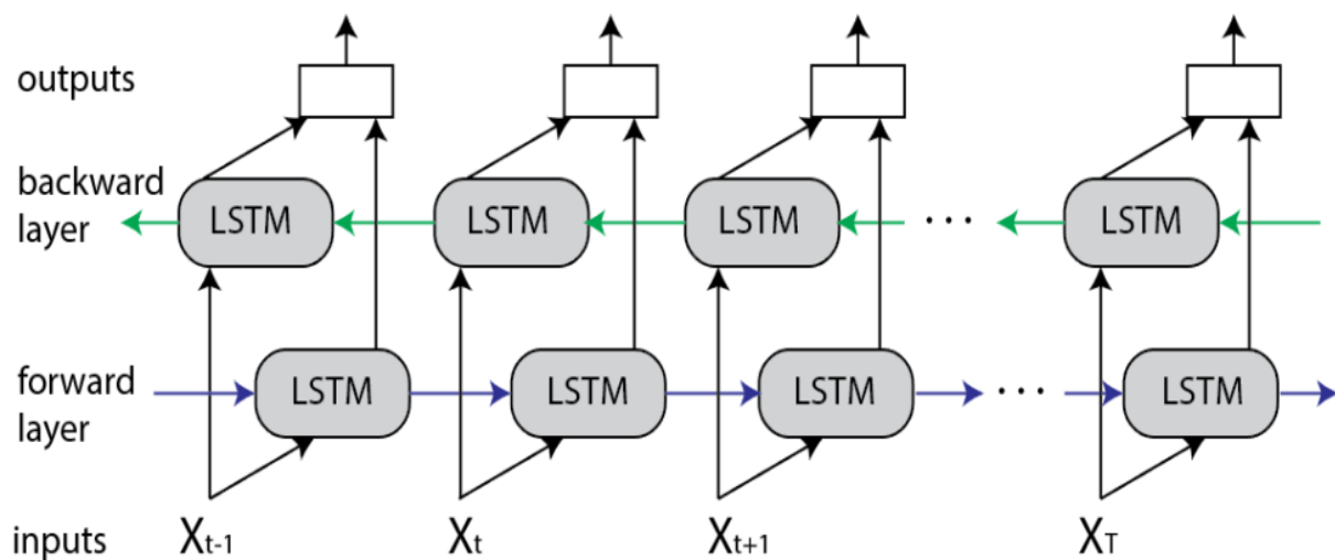
Figure 13. BiLSTM structure overview, [42].
