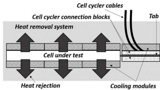
Figure 3: Schematic of test area within the assembly of the conductive thermal control apparatus
