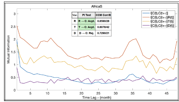
Figure 5: Sub-Saharan causal results of PI, CCM, and CMI by region. The abbreviations are: Var = variable, Acpt. = Acceptance, Rej. = Rejection, Corr = Correlation, RTS = Reconstruction Time Steps, C = Conflict, R = Rainfall, T = Temperature, D = Natural Disaster, R \Rightarrow C = R cause C.
