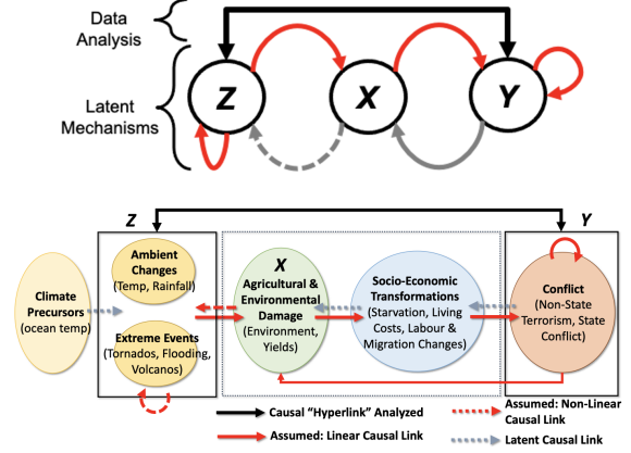
Figure 2: Our assumptions of the overall causal mechanisms between climate change, social transformation, and conflict. End-to-end causal data analysis (top) between Z and Y will be validated by artificial data generated by a causal toy model (bottom).
