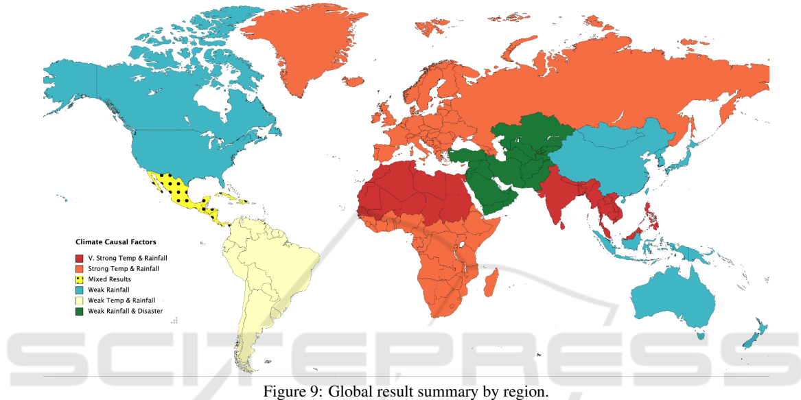
Figure 9: Global result summary by region.
