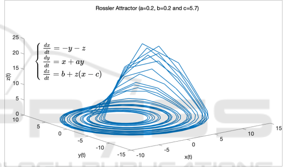
Figure 3: Rossler toy model and underlying equations and parameters.
