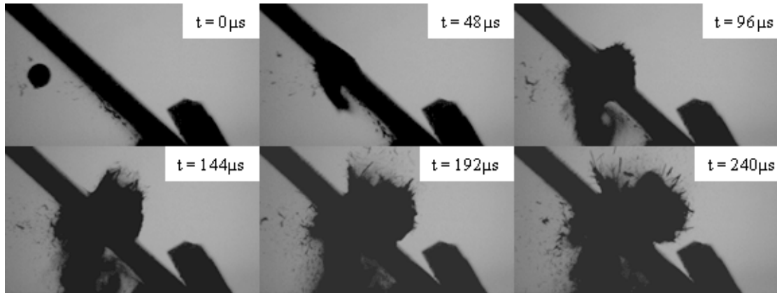
Figure 10: Perforation of a 12-mm thick two-part oblique laminate ; impact energy = 615 J (414 m/s). Here, the frame rate for the camera has been increased to 21,000 fps.
