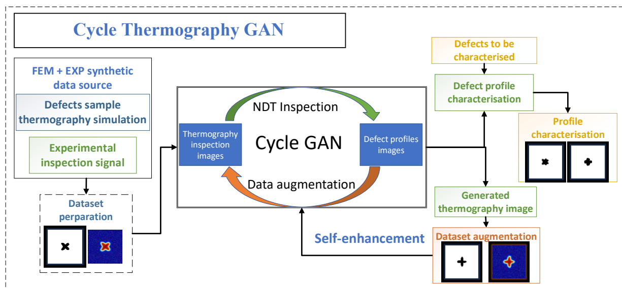
Figure 1. The proposed overall methodology
