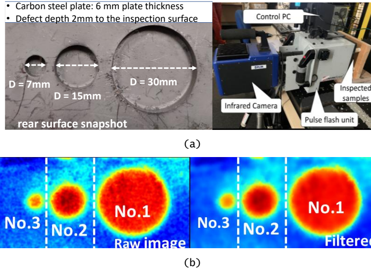
Figure 7. Experimental specimen and PT thermal images. (a) Defect specimen and PT experiment system; (b) Raw and pre-processed experimental data.
