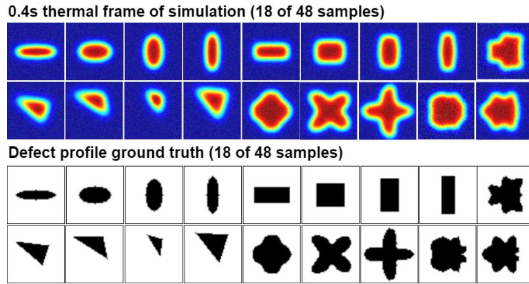
Figure 6. Simulation defects dataset
