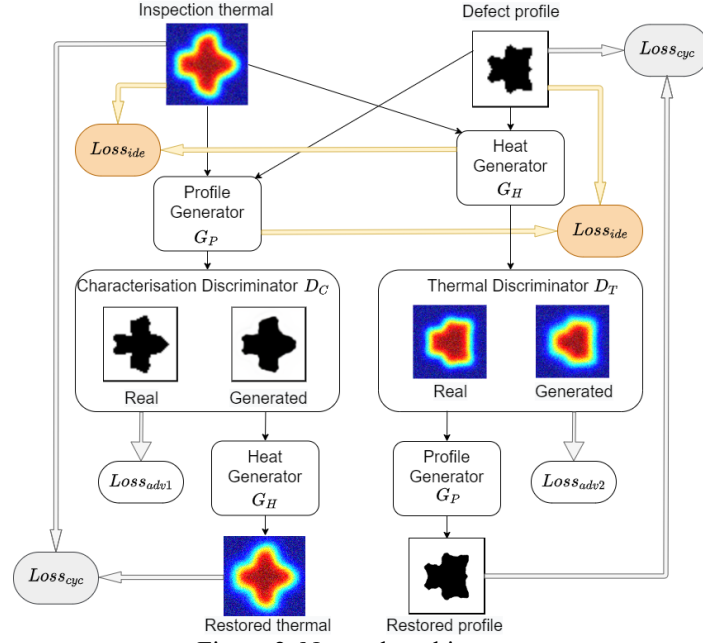
Figure 2. Network architecture
