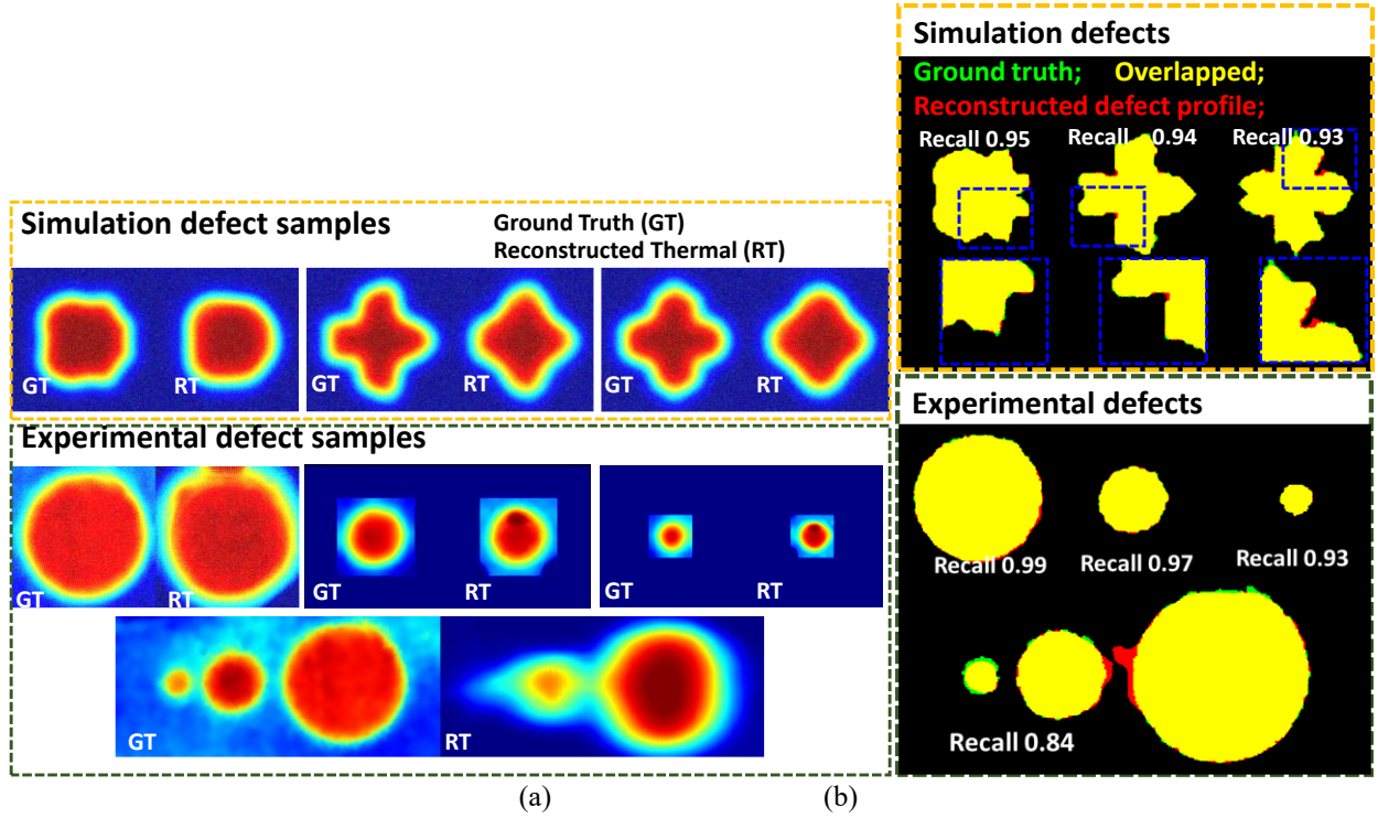
Figure 9. Comparison result using synthetic dataset. (a) Ground Truth (GT) and Reconstructed Thermal (RT) image; (b) Defect profiles overlap plot;
