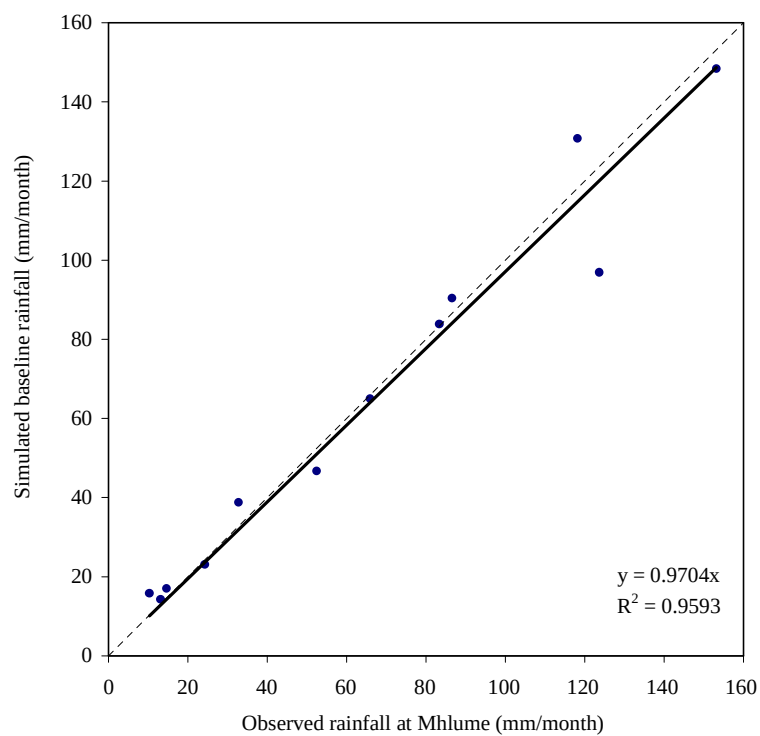
Figure 2 Comparison of observed mean monthly rainfall (mm/month) and mean daily (mm/day) reference evapotranspiration (ET o ) for Mhlume against simulated grid pixel data from the IWMI baseline climatology.
