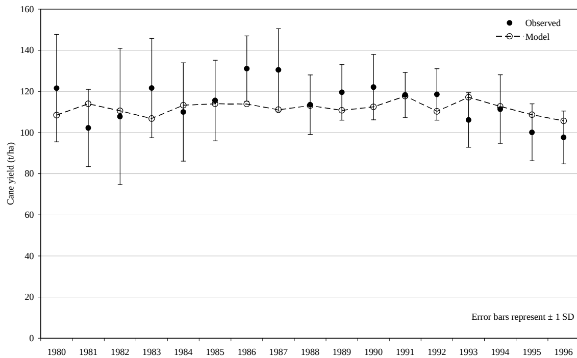
Figure 4 Comparison between CANEGRO simulated average annual yield (t/ha) and RSSC average annual field yield (observed) between 1980-1996.
