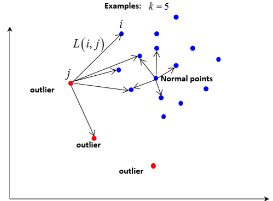
Figure 15. The illustration of k -nearest neighbor approach [6].
