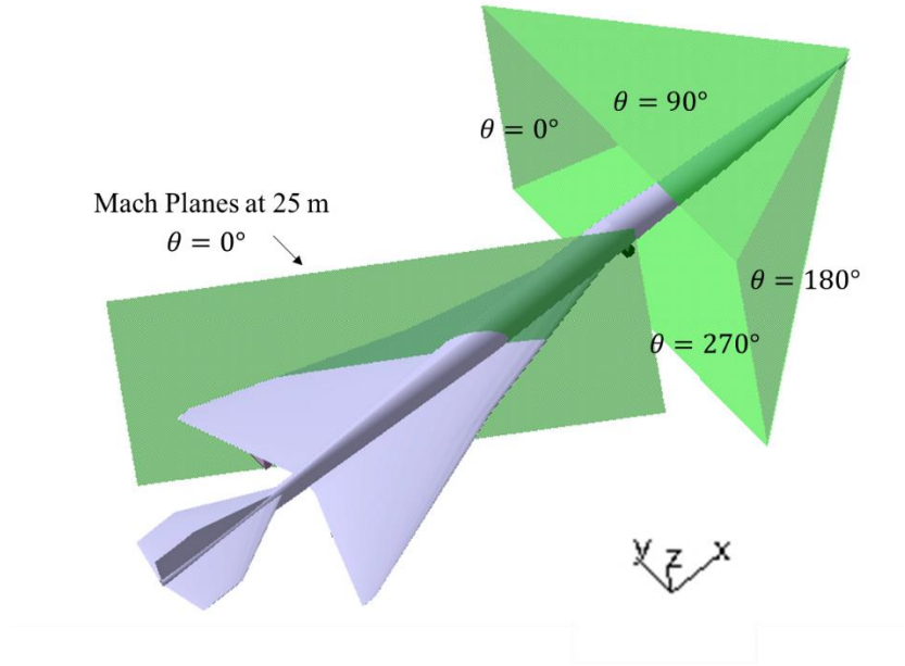
Fig. 5 Illustration of wave drag calculation procedure
