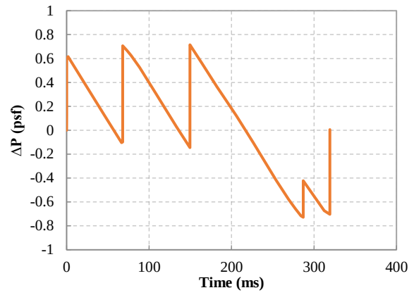
b. Low-boom optimization ground pressure
