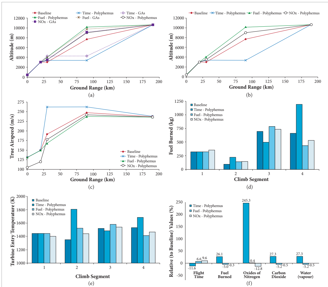
Figure 4. Case 2 – Implicitly constrained climb profile optimisation results.
