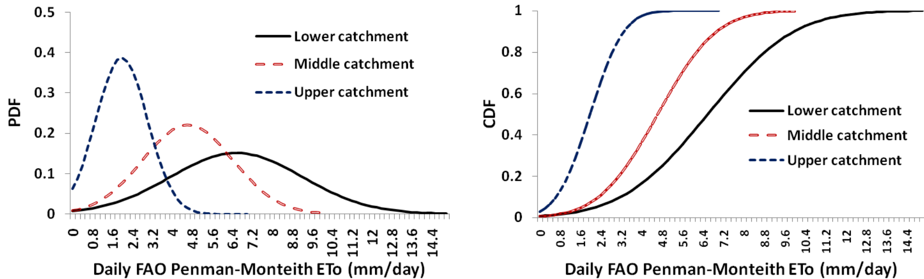
Figure 2: The PDF and CDFs of reference evapotranspiration for three sub-catchments calculated using National Centres for Environmental Protection (NCEP) Climate Forecast System Reanalysis (CFSR) data
