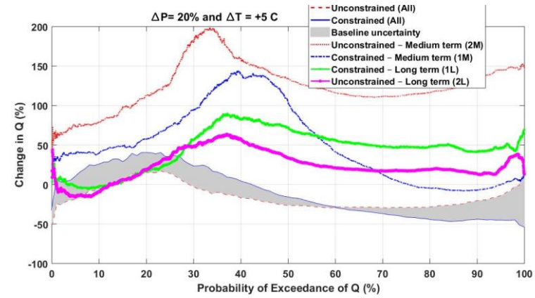
Figure 9: Comparison of medium and long term future impact uncertainty (as given by the percentage change in daily discharge [compared to \Delta T = 0^\circ\text{C} , \Delta P = 0\% ] across the flow exceedance probability for four selected change factor scenarios for the two models) and their baseline model uncertainty. N:B. We have used notations like 1M, 2M, 1L and 2L etc for denoting different models with medium term and long term assumptions.
