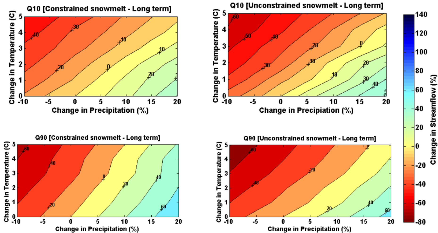
Figure 8: Impact Response Surfaces of the change in simulated (upper) Q10 and (lower) Q90 daily discharge under changed annual temperature and precipitation for long term future conditions with no permanent snow/icepack for models with contrasting baseline snow/ice pack behaviour assumption
