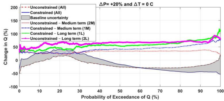
Figure 9: Comparison of medium and long term future impact uncertainty (as given by the percentage change in daily discharge [compared to \Delta T = 0^\circ\text{C} , \Delta P = 0\% ] across the flow exceedance probability for four selected change factor scenarios for the two models) and their baseline model uncertainty. N:B. We have used notations like 1M, 2M, 1L and 2L etc for denoting different models with medium term and long term assumptions.
