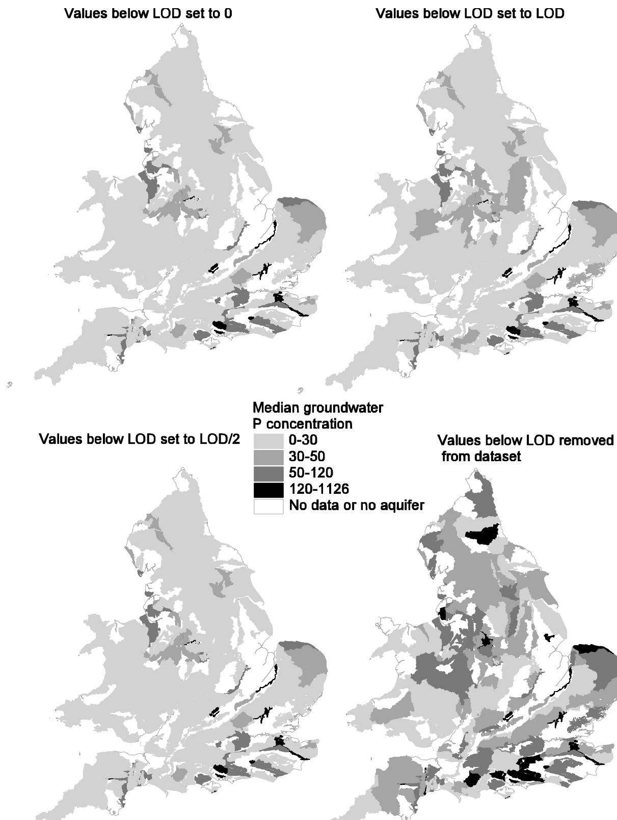
Figure 2 Effects of the treatment of samples below LOD on median groundwater P concentration ( \mu\text{g P l}^{-1} ) in the groundwater bodies of England and Wales
