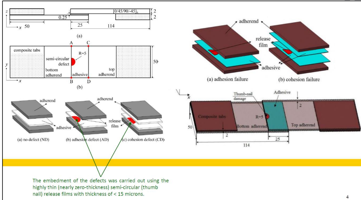
Figure 14: Artificial defects release film kissing bond [25].
