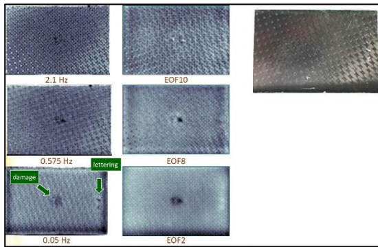
Figure 5: Sample A4 (15 J woven), front face (impacted side), PPT and PCT. The damage is barely visible in the original image of the composite (Far right image), the white marks are lettering from labelling the specimen. The 0.05Hz PPT image, shows clear subsurface damage [5].
