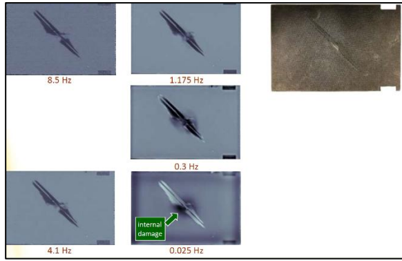
Figure 9: Sample 20 J Demo, Reflection rear face. PPT. The rear face has some substantial damage. The PPT locates the surrounding internal damage [5].
