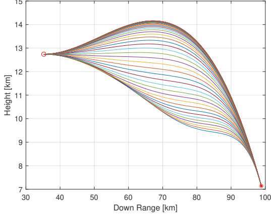
(a) Trajectory of the missile (Case 3).
