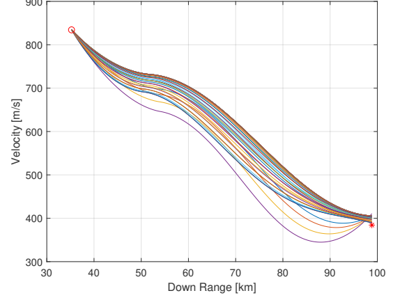
(b) Velocity of the missile (Case 1).
