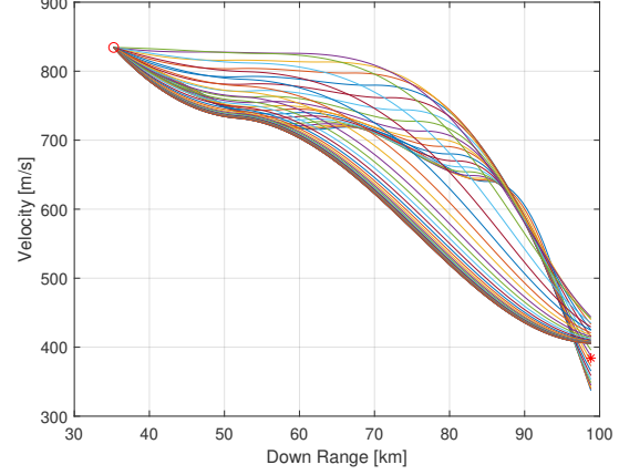
(b) Velocity of the missile (Case 3).
