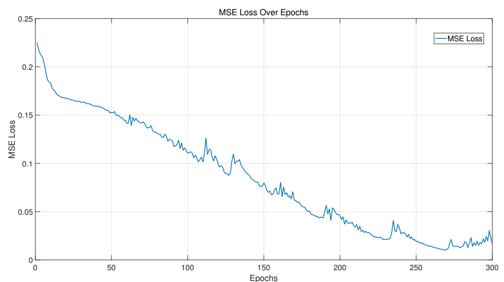
Figure 38. MSE loss during training.
