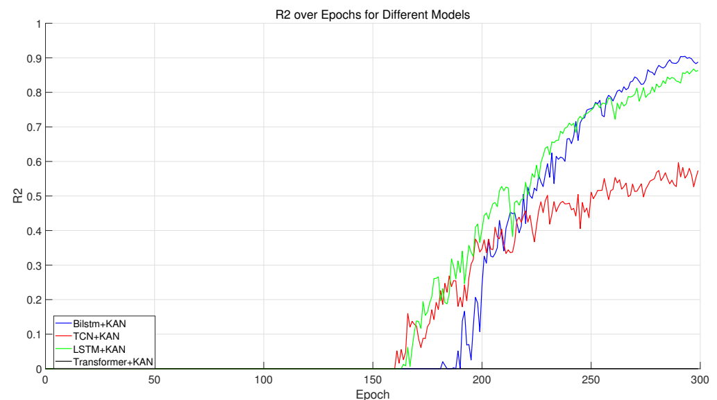
Figure 44. R^2 over epochs for different models (TCN, LSTM, and transformer) with KAN.
