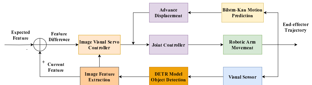
Figure 13. Visual servo simulation flowchart.
