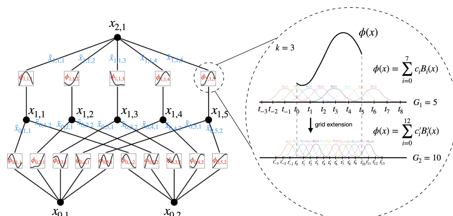
Figure 12. Basic architecture diagram of KAN—Ziming Liu et al. [46].
