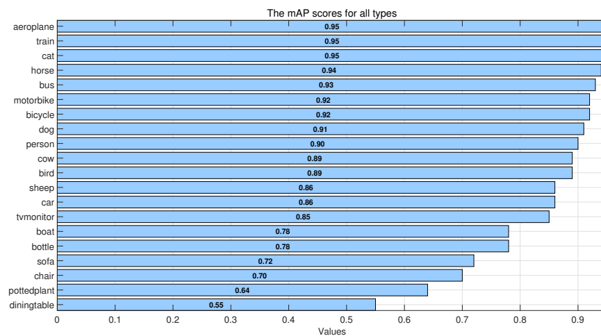
Figure 22. The mAP scores for all types.
