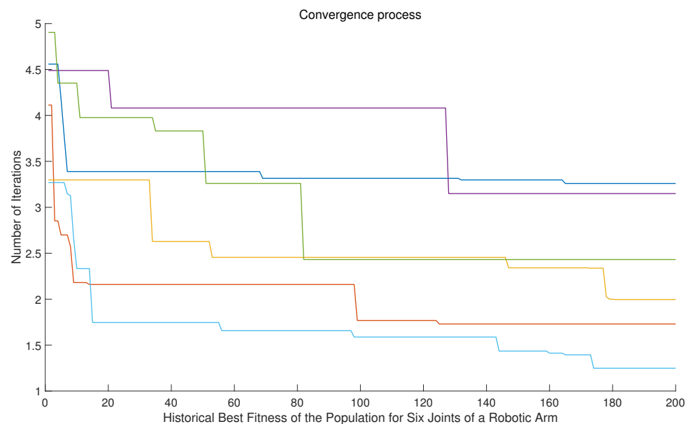
Figure 36. The change chart of the best fitness in population history.
