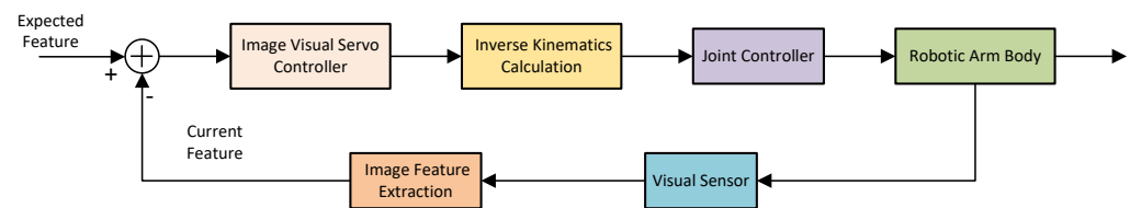
Figure 1. Image-based visual servoing flowchart.
