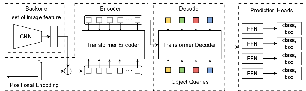
Figure 7. DETR structure diagram.
