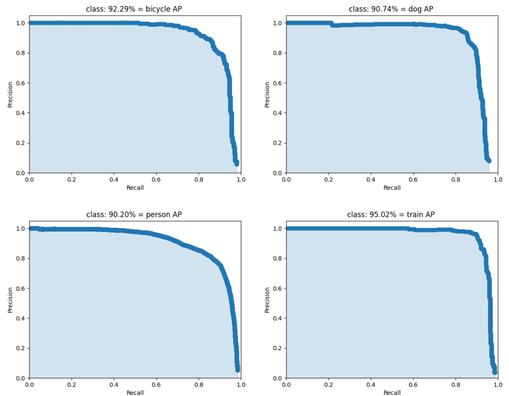
Figure 21. AP scores for bicycle, dog, person, and train.
