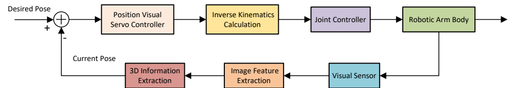
Figure 2. Position-based visual servoing flowchart.
