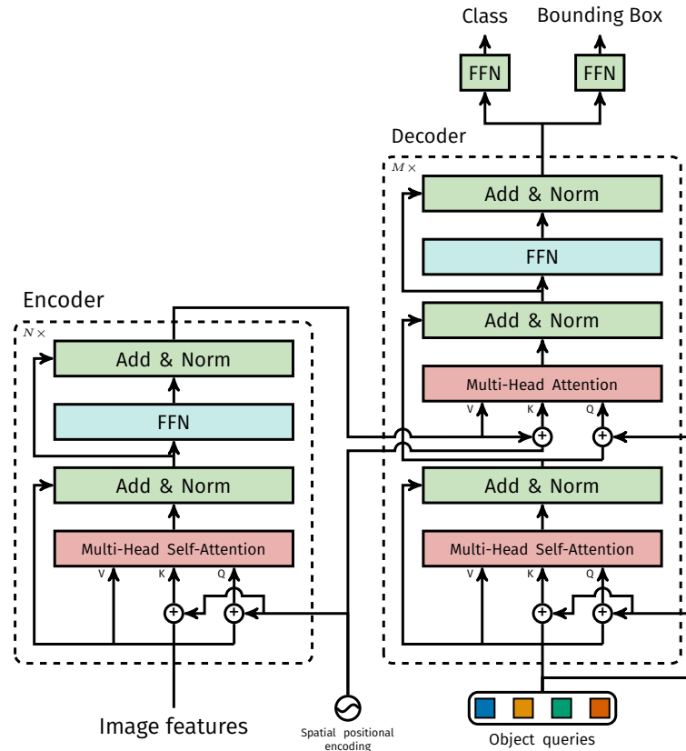
Figure 6. The architecture of DETR's transformer [44].
