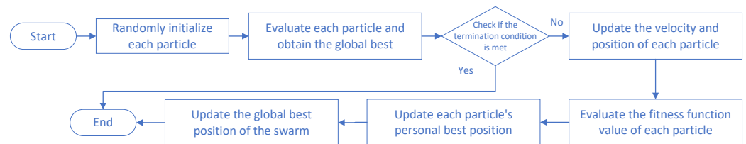
Figure 8. PSO algorithm flow.
