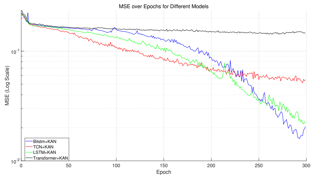
Figure 43. MSE over epochs for different models (TCN, LSTM, and transformer) with KAN.
