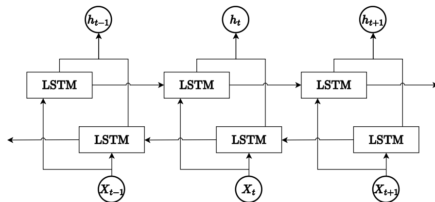
Figure 10. BiLSTM structure diagram.
