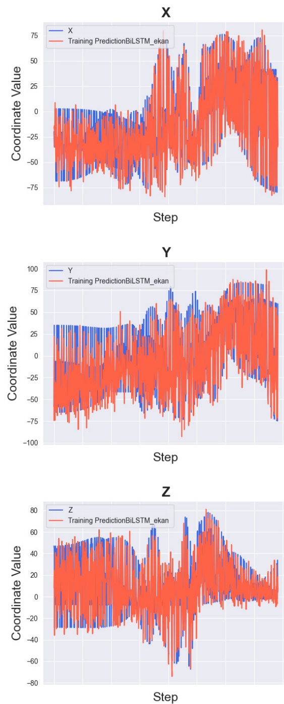
Figure 45. Training predictions for BILSTM with KAN on X, Y, and Z coordinates.
