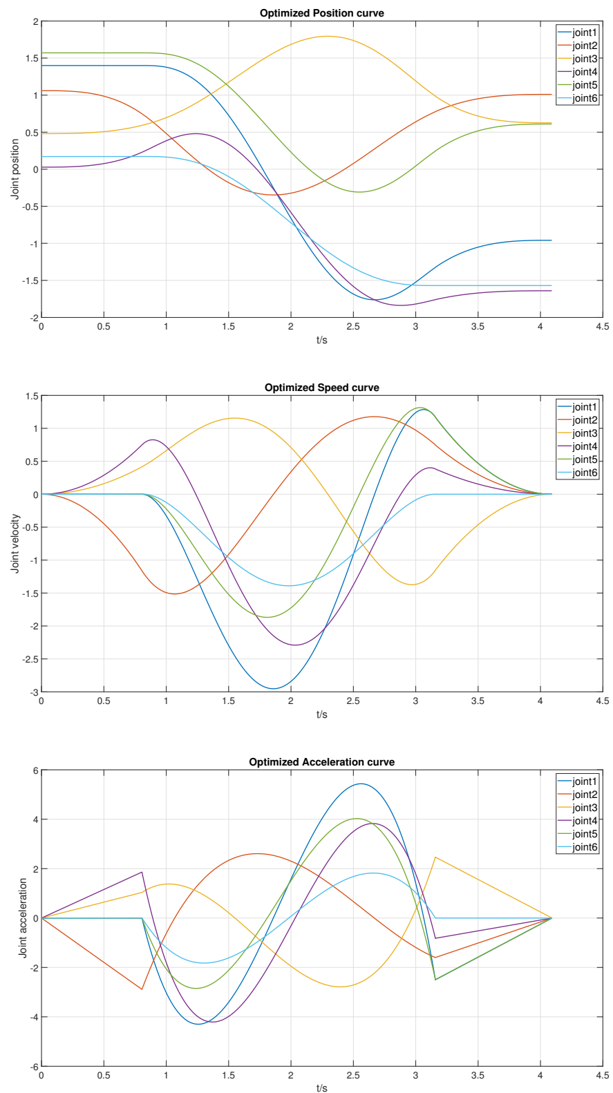
Figure 37. The comparison before and after PSO algorithm optimization.
