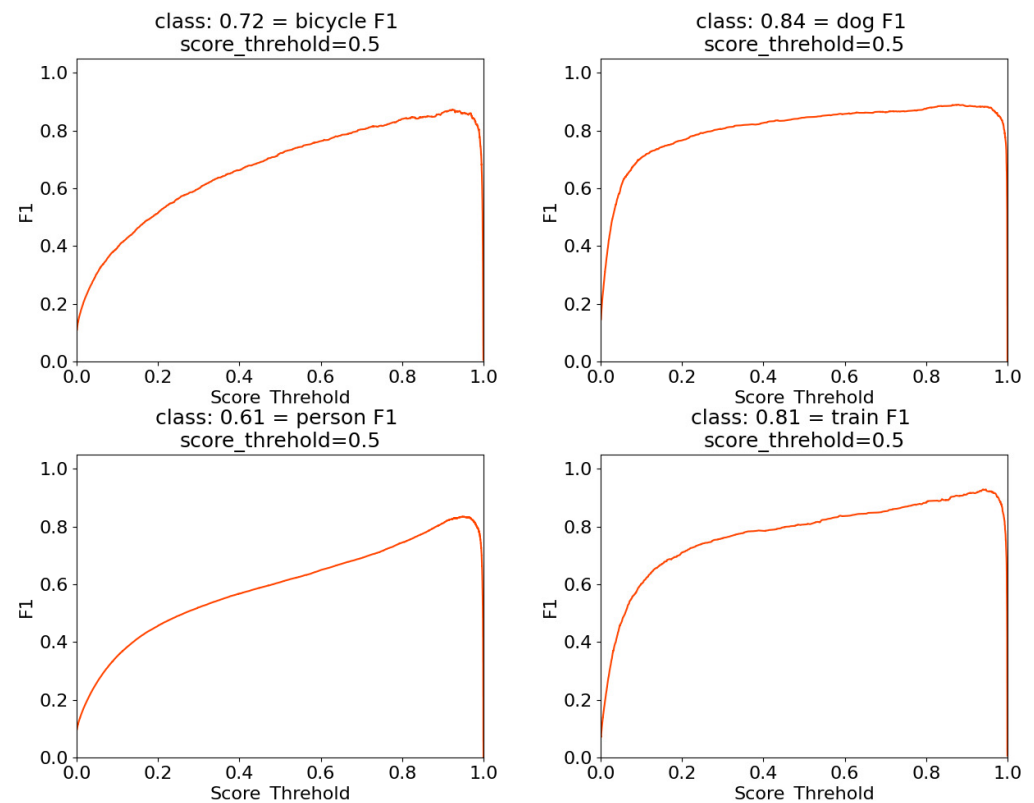
Figure 23. F_1 scores for bicycle, dog, person, and train.
