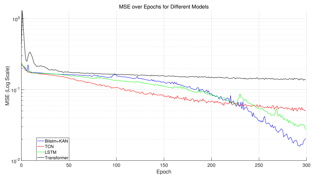
Figure 41. MSE over epochs for different models (TCN, LSTM, and transformer).
