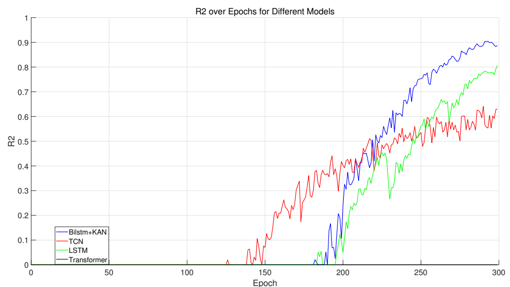
Figure 42. R^2 over epochs for different models (TCN, LSTM, and transformer).
