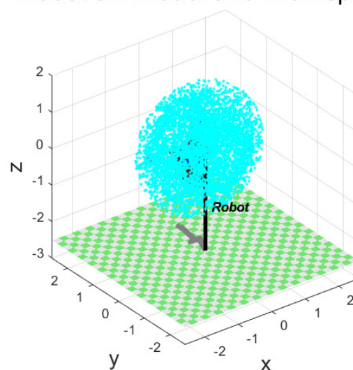
Figure 34. Robot arm 3D model and workspace.
