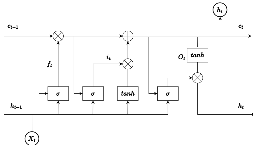
Figure 9. LSTM unit structure diagram.
