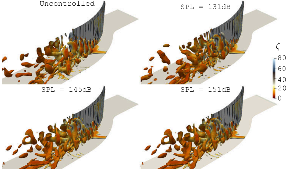
Fig. 14 The effect of excitation amplitude on the iso-surfaces of Q-criterion at Q = 10^9 coloured by \Omega^* .
