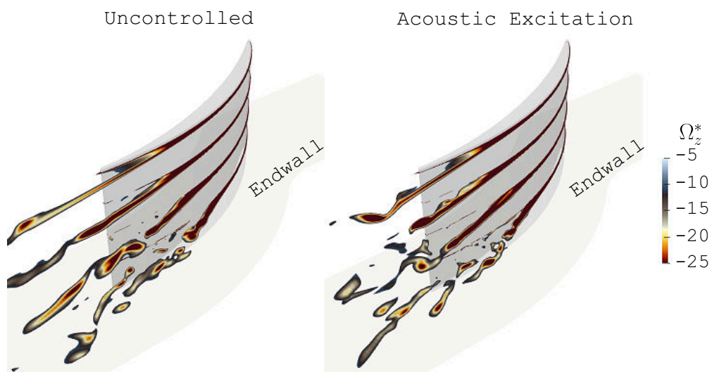
Fig. 6 3D view of \Omega_z^* at spanwise stations.
