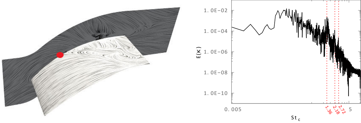
Fig. 3 Surface flow topology and the monitor location (left) and turbulent kinetic energy spectrum at the onset of corner flow separation (right).
