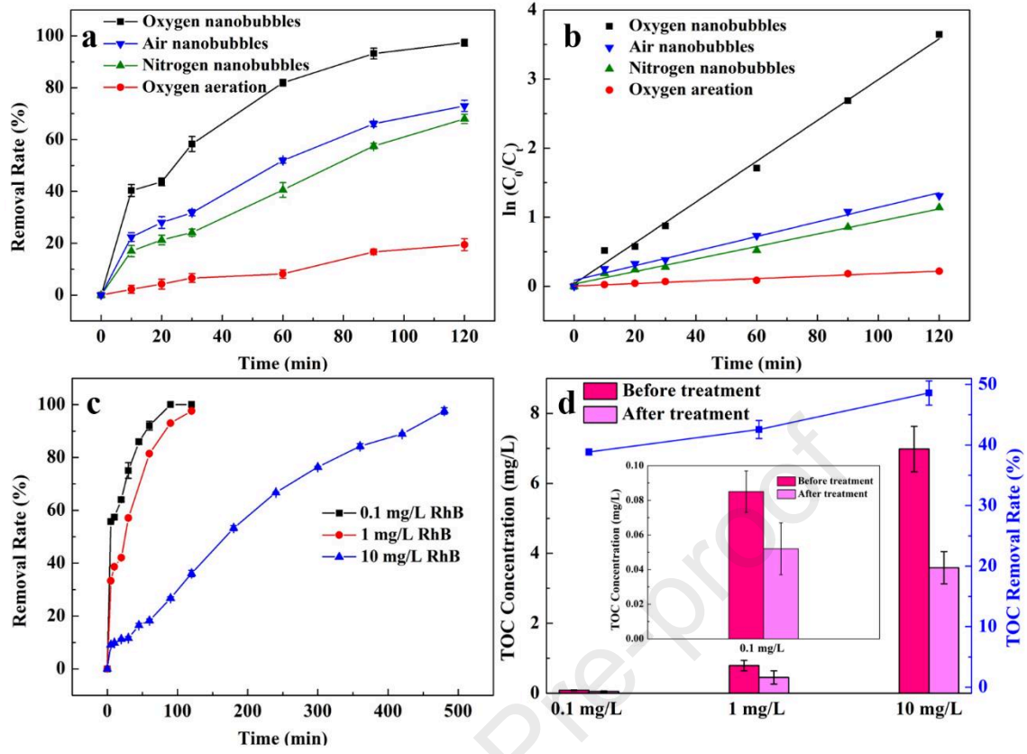
Fig. 2. The remove rates of RhB at an initial concentration of 1 mg/L for water treated by oxygen, air and nitrogen nanobubble, and conventional oxygen aeration process (a), as well as the fitted first-order kinetics model (b), the removal rate of RhB by oxygen nanobubble treatment for different RhB initial concentrations (c), the initial and final concentrations of TOC in all treatment groups (d).
