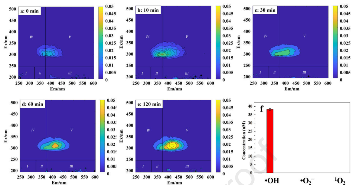
Fig. 4. Excitation and emission matrix (EEM) fluorescence spectra of oxygen nanobubble water in the presence of the fluorescent probe at different times (a-e) and the concentrations of ROSs generated in the experimental system (f).
