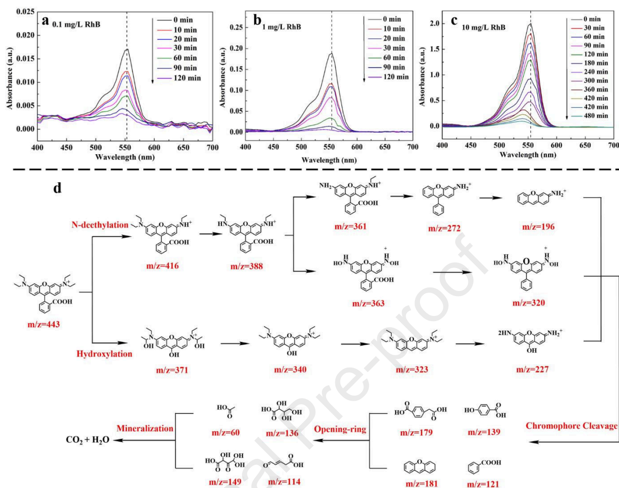
Fig. 5. UV-vis absorption spectral variations for RhB at different reaction times for initial dye concentrations of 0.1 (a), 1 (b), and 10 (c) mg/L; the potential degradation pathway of RhB by oxygen nanobubbles (d).
