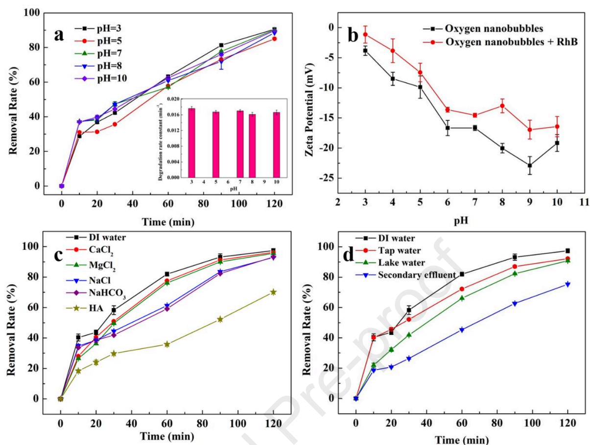
Fig. 6. The removal efficiencies of RhB at an initial concentration of 1 mg/L by oxygen nanobubble treatment under initial pH levels of 3-10 (a), the Zeta potential of oxygen nanobubbles before and after reacting with RhB (b), the removal efficiencies of RhB at an initial concentration of 1 mg/L in the presence of different background ions and organic matter (humic acid – HA) by oxygen nanobubble treatment (c) and removal in different real water samples by oxygen nanobubble treatment (d).
