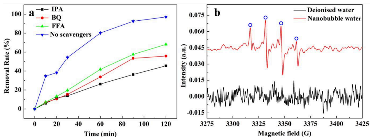
Fig. 3. Effect of scavengers on the degradation of RhB at an initial concentration of 1 mg/L (a), ESR evidence for \bullet\text{OH} production from oxygen nanobubbles (b).
