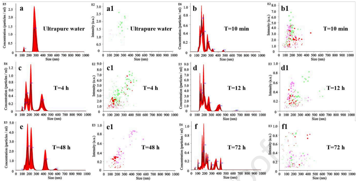
Fig. 1. The size and distribution of nanobubbles in ultrapure water (a) and the prepared nanobubble water at 10 min (b), 4h (c), 12h (d), 48h (e), and 72h (f). The operation time of the generation was 10 mins. Different colours in the intensity/size graphs (a1-f1) represent the results from three separate measurements.
