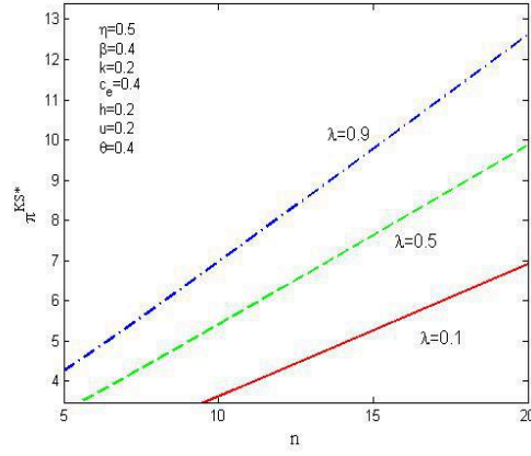
Figure 5: The impact of n on \pi_i^{KS*}
