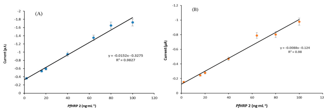
Figure 5. Linear regression analysis of the chronoamperometric response of Pf HRP 2 detection in buffer (PBS, 0.01\text{M} , pH 7.4, spiked with 1\text{--}100 \text{ ng}\cdot\text{mL}^{-1} Pf HRP 2) (A) and 100% serum samples (spiked with 1\text{--}100 \text{ ng}\cdot\text{mL}^{-1} Pf HRP 2) (B) on a JD2 sensor. Measurements were conducted at -0.2 \text{ V} . Correlation coefficient and R^2 value of 0.9827 for the buffer matrix and 0.98 for the serum matrix ( n = 3 ).
