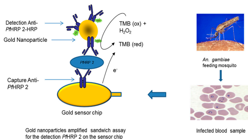
Scheme 1. Principle of the developed sensor for malaria detection.
