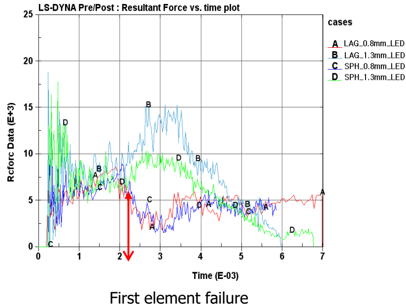
Figure 14. Force vs time history plot for both Lagrangian (LAG) and SPH models.
