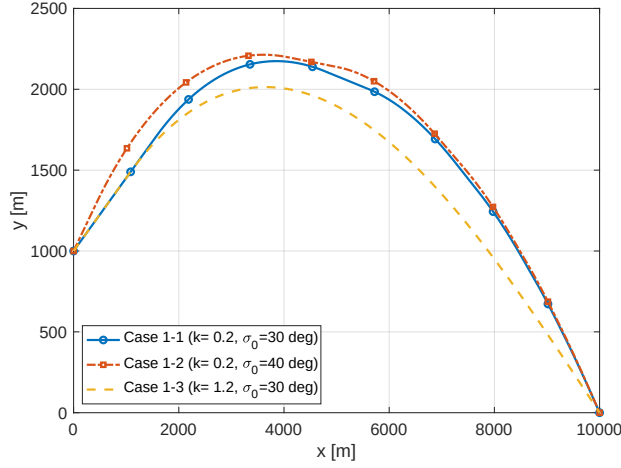
(a) Trajectory
