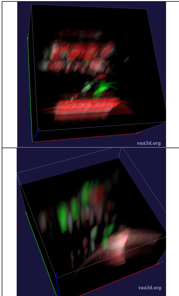
Figure 3-5 , 3D polarimetric SAR images of the mock building scene. Radar down-range is aligned up the page with the green y-axis. The image is colourized according to Odd (red) and Even (green) bounce scattering, parametrized by the modulus of the Skip parameter. The top image is monostatic, whereas the bottom image is bistatic, with a fixed receiver to the right of the scene.
