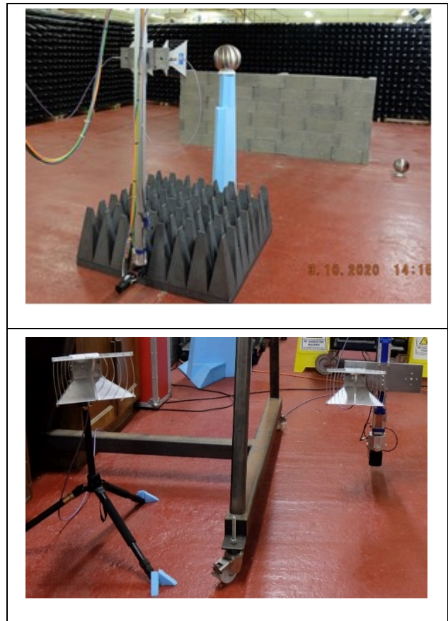
Figure 3 1 , Microwave antennas in monostatic configuration undergoing calibration (top), and in bistatic configuration (bottom).
