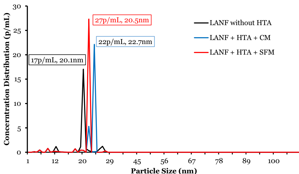
Fig. 6 Experimental result of particle size and concentration distribution measurement for alumina nanoparticles in the three samples using NanoSight NS300
