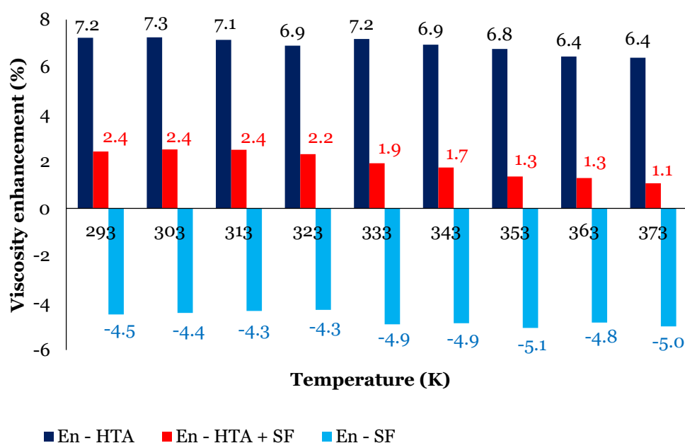
Fig. 11 Calculated results of dynamic viscosity enhancement (%) of samples against temperature (K). Where En-HTA + SF is enhancement due to HTA addition and surface functionalisation; En-HTA is enhancement due to HTA addition; and En-SF is enhancement due to surface functionalisation
