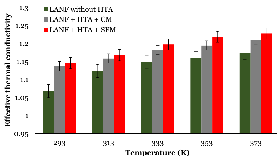
Fig. 8 Calculated results of effective thermal conductivity of samples against temperature (K) using Eq. 1
