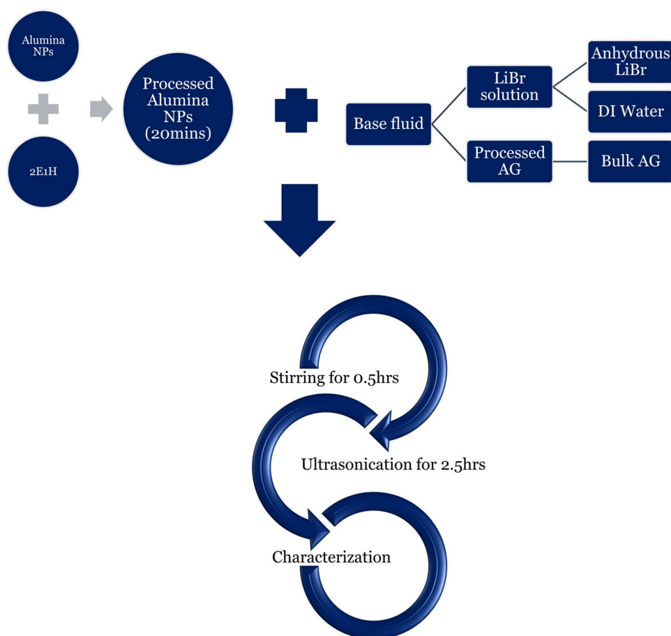
Fig. 2 Schematic flow chart for a new synthesis procedure of nanofluid with HTA
