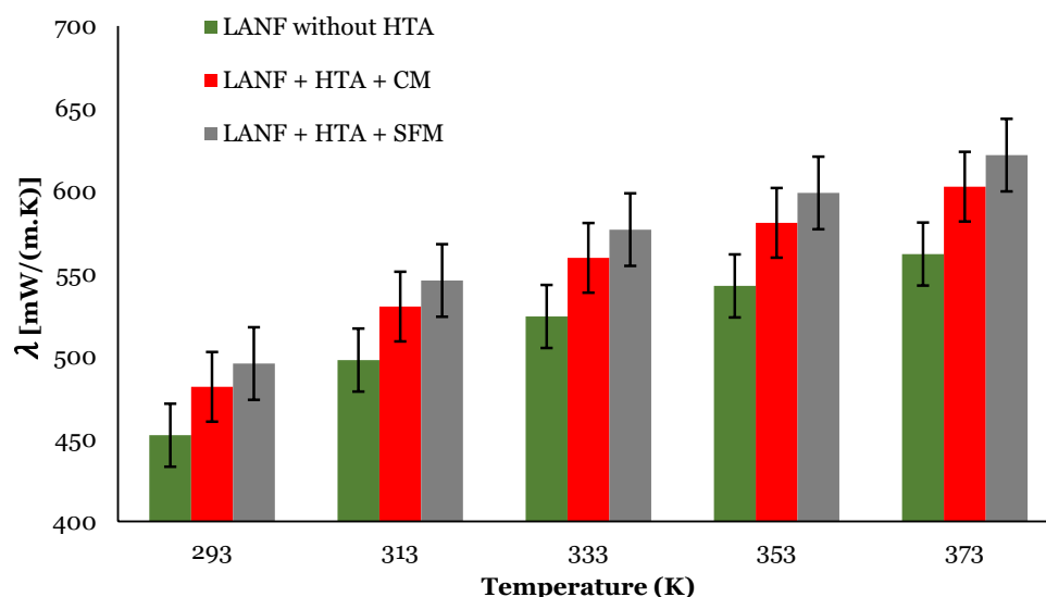
Fig. 7 Experimental results of thermal conductivity of samples against temperature (K)
