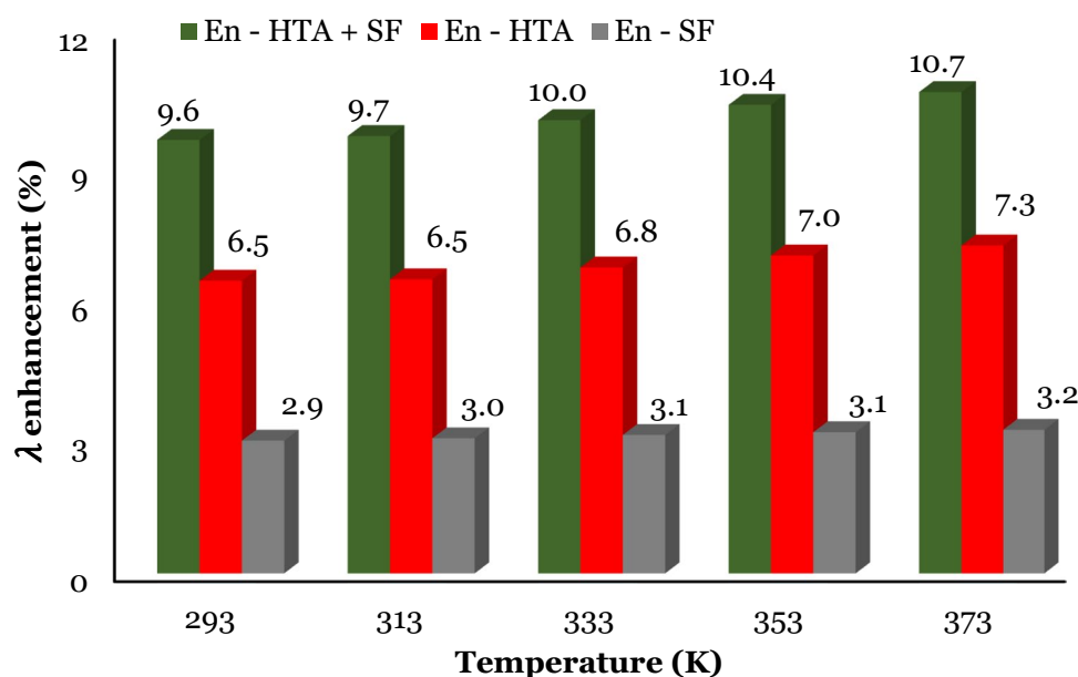
Fig. 9 Calculated results of thermal conductivity enhancement (%) of samples against temperature (K). Where En-HTA+SF is enhancement due to HTA addition and surface functionalisation; En-HTA is enhancement due to HTA addition; and En-SF is enhancement due to surface functionalisation
