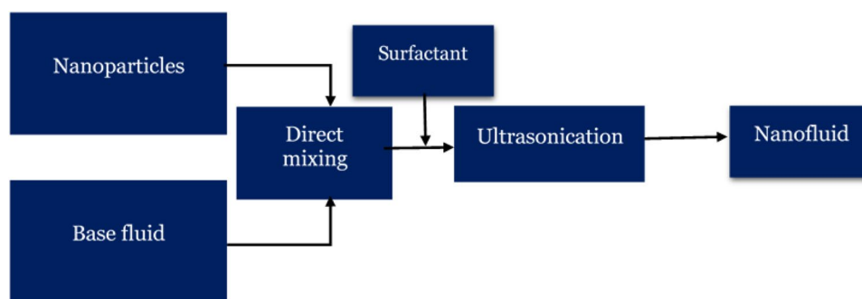
Fig. 1 Schematic of a conventional procedure for binary nanofluid synthesis with a surfactant using a two-step method [31]. Direct mixing with magnetic stirrer at 400 rpm for 2 h, and ultrasonication for up to 7 h is usual conventional practice. In both cases, temperatures are maintained between 298 and 308 K
