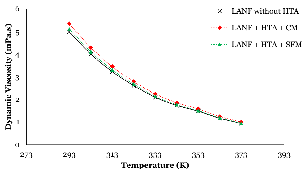
Fig. 10 Experimental results of dynamic viscosity of samples against temperature (K) at 2\text{S}^{-1} shear rate and \pm 1\% standard error
