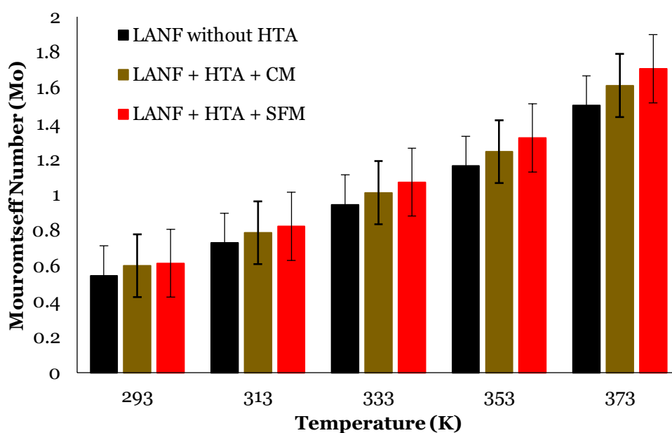
Fig. 12 Calculated results of Mouromtseff Number ( Mo ) against temperature using Eq. 5 for LANF sample without HTA, LANF with HTA prepared by conventional method (CM) and LANF with HTA prepared by surface functionalisation method (SFM)
