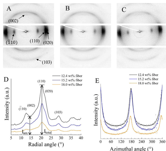
Figure 7. Typical WAXD patterns of (A) 12.4, (B) 15.2, and (C) 18.0 wt % cellulose fibers, as well as their (D) radial scanning data and (E) azimuthal scanning data from the (110) peak.
