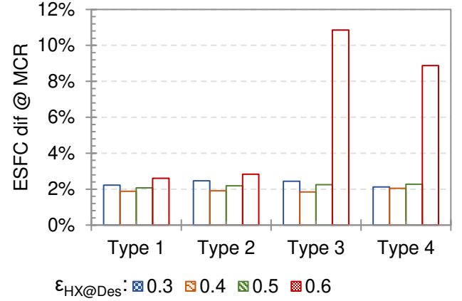
FIGURE 18: ESFC difference compared to the respective baseline engine performance over varying heat exchanger designs and engine types
