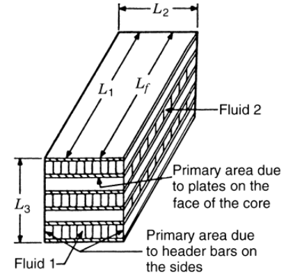
FIGURE 5: Plate-fin heat exchanger – Crossflow [18]
