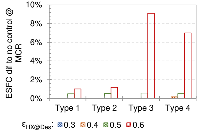
FIGURE 19: ESFC difference with and without T_{HX,Hot,out} control
