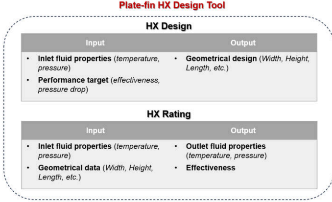
FIGURE 7: Plate-fin heat exchanger design tool
