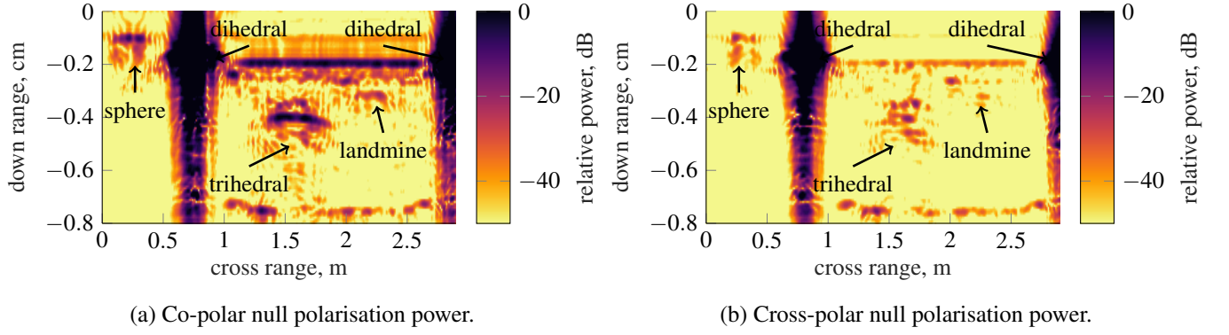
Figure 8. Bscan images for the P_{co} co- and P_x cross-polar null polarisation filtered powers (compare with Figs 3-5).
