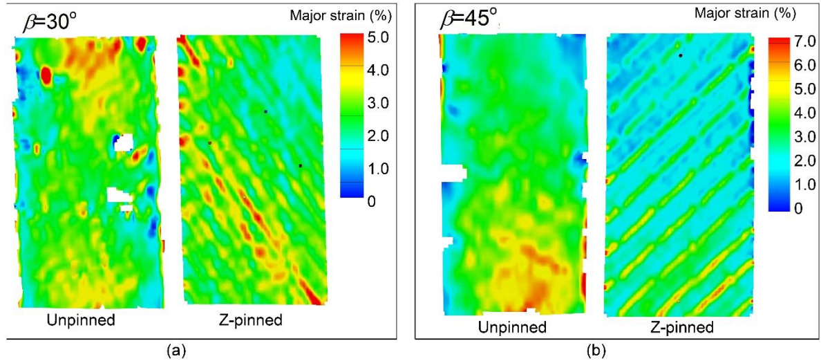
Fig.9 (a) major strain field at the axial strain of 0.032 for off-axis angle of 30°; (b) major strain field at the axial strain of 0.045 for off-axis angle of 45°;
