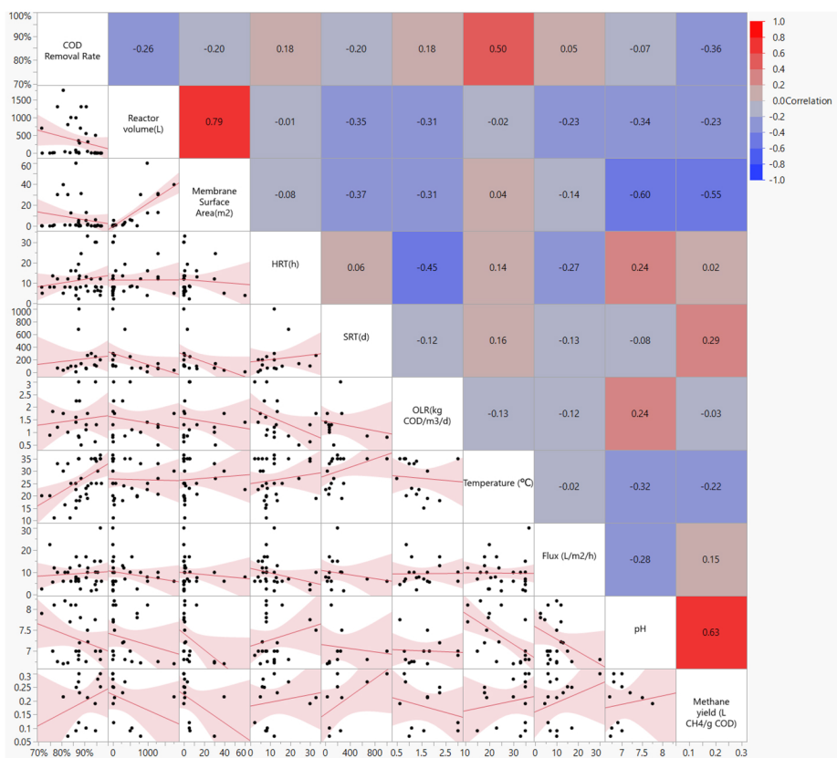
Figure 3. Multivariate correlations scatterplot matrix of operational parameters.
