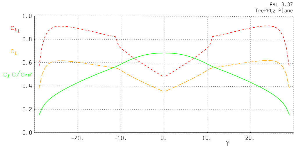
Fig. 5 Lift distribution along the span. Cruise condition.
