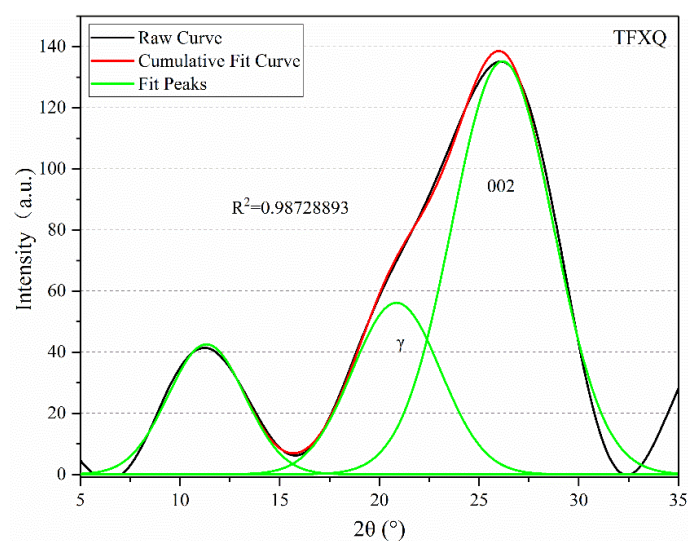
Fig. 2 Gaussian fitting curve of \gamma peak and 002 peak of TFXQ coal sample in 2\theta range of 5-35° From the results of peak fitting, we can obtain the area of the 002 peak and \gamma peak, and thus the
