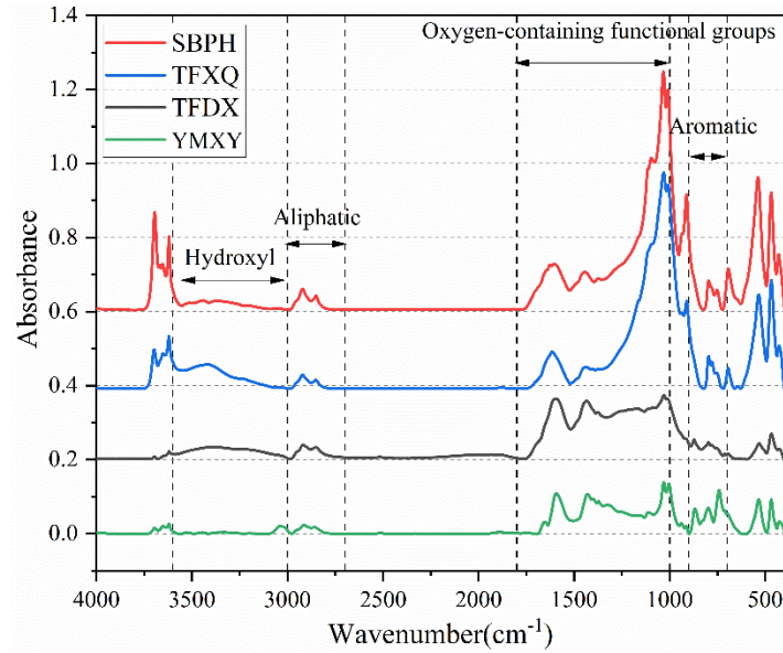
Fig.5 FTIR spectra of four coal samples
