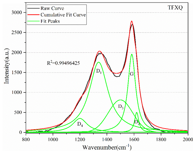
Fig. 4 Raman spectrum of TFXQ coal with the corresponding curve fitted bands Positions of G peak and D_1 peak, difference of peak position (G- D_1 ), and integrated intensity ratio ( I_{D1}/I_G ) and other characteristic parameters are important parameters for evaluating the degree of crystallinity or degree of defects in carbonaceous materials. The output data is shown in Table 3. It can be seen from Table 3 that the peak positions of the G and D_1 peaks of the four coal samples are
