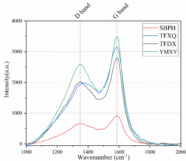
Fig. 3 The Raman spectra of four coal samples
