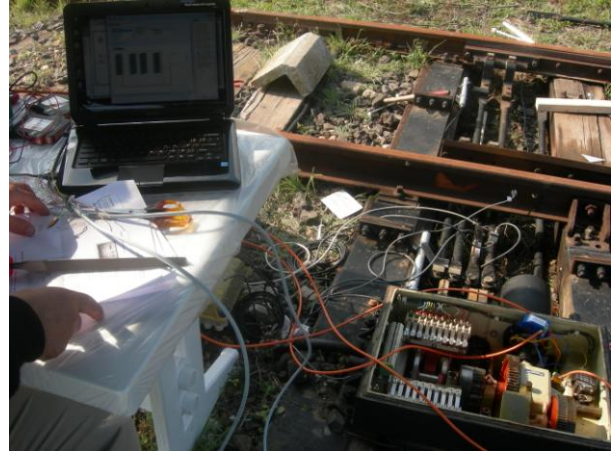
Fig 2: Railway turnout system with sensors installed
