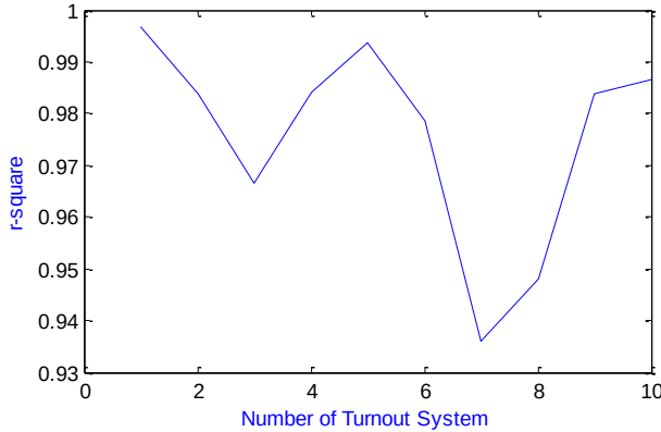
Fig 9: r-square values of estimated and real RUL for ten turnout systems
