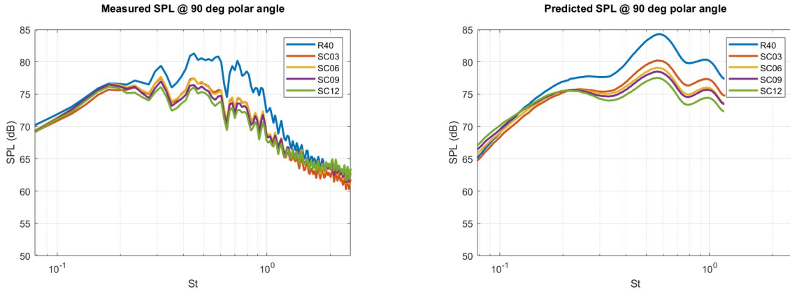
Fig. 14 Measured and predicted installed Sound Pressure Levels for all nozzles at \theta = 90^\circ - M_f = 0.1
