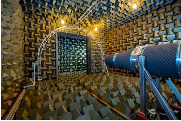
(a) Far-field measurements
