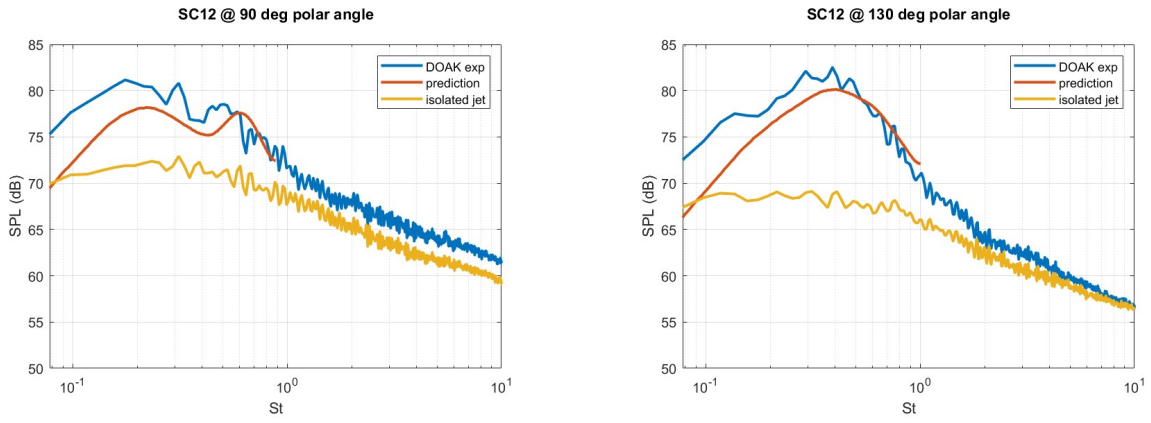
Fig. 6 Installed noise predictions versus experiments for nozzle SC12 - static case
