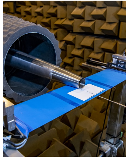
(c) Flowfield measurements
