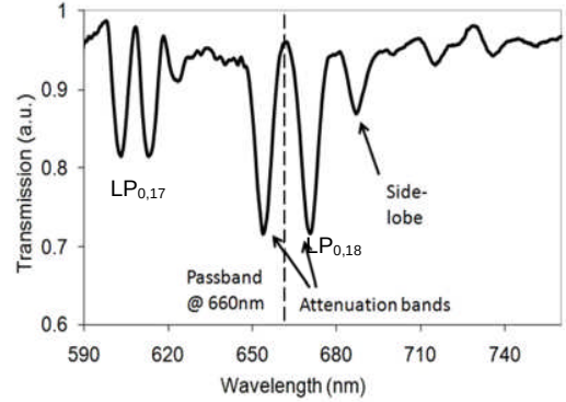
Fig. 3. The transmission spectrum obtained from a length-apodized phase-shifted LPG of period 100 μm and length 27mm. The two attenuation bands that characterize the coupling to each cladding mode are the result of the phase shifts created within the LPG. The side-lobe indicated is a known by-product of length apodization [8].
