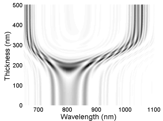
Fig. 8. Output from a numerical model of the response of the \text{LP}_{019} resonance of a length-apodized phase-shifted LPG to the deposition of a coating onto sections 2, 4, 5 and 6 (as identified in figure 2). The period of the LPG, 100 \mu\text{m} , is such that the resonance is at its phase matching turning point. The grey scale relates to the transmission, with black representing the lowest transmission white represents the maximum transmission
