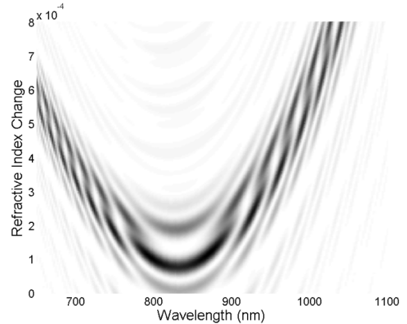
Fig. 10. Numerically modeled response of the LP_{0,19} mode resonance feature of a length-apodized phase-shifted LPG to changes in the effective refractive index of the cladding mode in regions (4,5,6). The period of the LPG, 100\ \mu\text{m} , is such that the LP_{0,19} mode is at its phase matching turning point. The grey scale relates to the transmission, with black representing the lowest transmission white represents the maximum transmission
