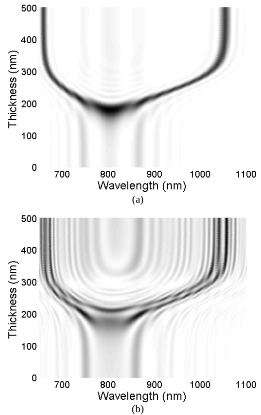
Fig. 7. Output from numerical model of the response of the \text{LP}_{019} resonance of (a) an LPG containing a single phase shift located at its centre the deposition of a coating over one half of the length of the LPG and (b) a length-apodized phase-shifted LPG to the deposition of a coating over sections 4,5 and 6 (as defined in figure 2). The period of the LPG, 100 \mu\text{m} , is such that the resonance is at its phase matching turning point. The grey scale relates to the transmission, with black representing the lowest transmission white represents the maximum transmission.
