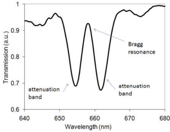
Fig. 1. Experimental transmission spectrum of a phase-shifted LPG of period 100μm and length 27mm, with a single \pi phase step located at the centre of the LPG. Attenuation bands located on either side of the resonance wavelength can be seen.
