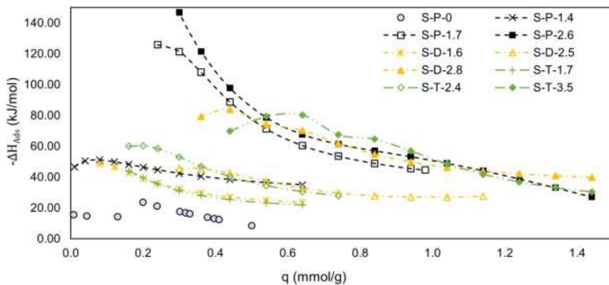
Figure 7. Isosteric heat of adsorption for raw SBA-15 and functionalised samples
