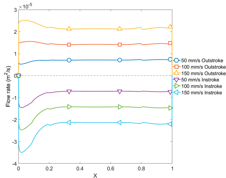
Figure 26. Flow rate per unit circumferential length at different piston velocities in the instroke and outstroke motion. Isotropic asperities and sealed pressure of 10 MPa.
