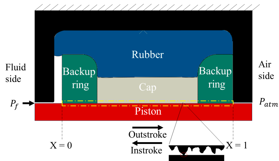
Figure 4. Fluid film channel enclosed by yellow line, and boundary conditions for mixed-EHL solution. Characteristic length for non-dimensional dimension X .
