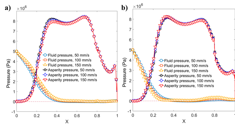
Figure 16. Fluid film pressure and asperity contact pressure distributions at different piston speeds at 5 MPa of sealed pressure: (a) Outstroke, (b) Instroke.
