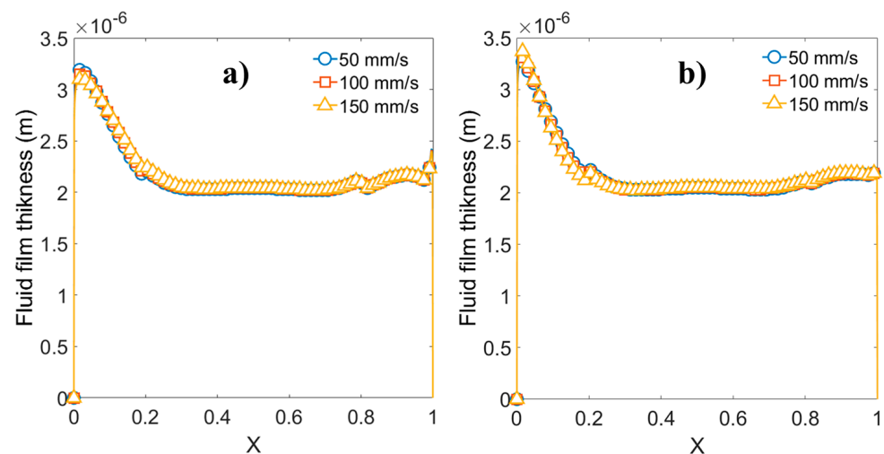
Figure 17. Fluid film thickness at different piston velocities in the instroke (a) and outstroke (b) directions. Sealed pressure: 5 MPa.
