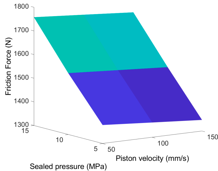
Figure 20. Variation in friction force with sealed pressure and piston velocity in the outstroke direction with isotropic asperities ( \gamma = 1 ).
