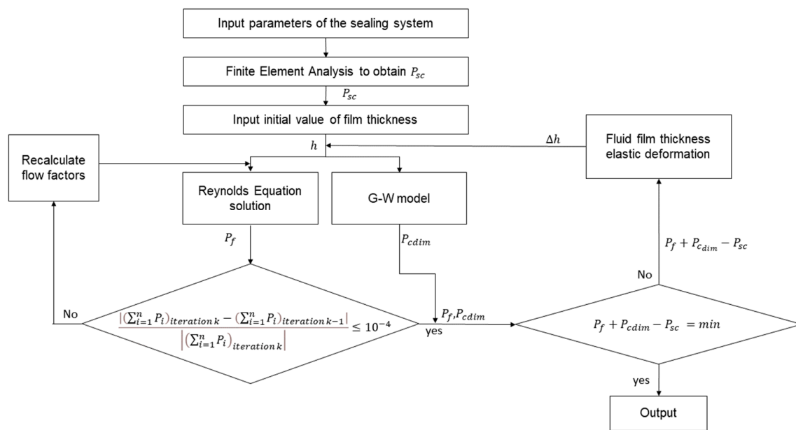
Figure 7. Computational process.
