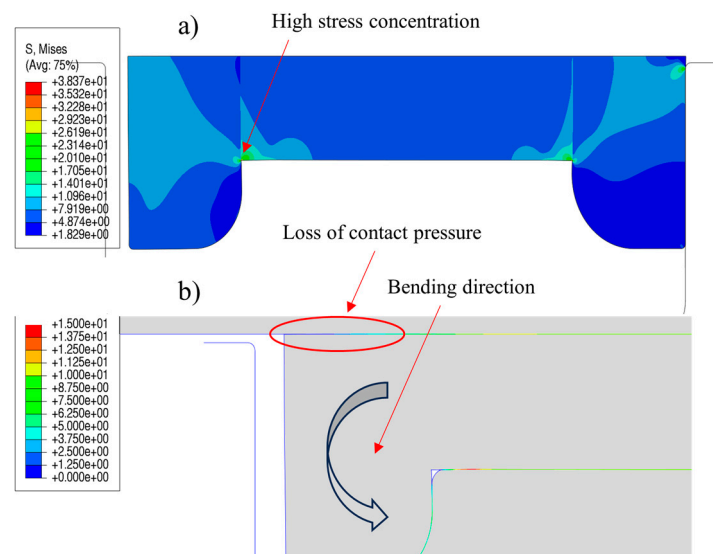
Figure 13. Loss of contact pressure in the vicinity of X = 0 due to part deformation at 10 MPa of sealed pressure. (a) Von Mises stress of the part comprising the backup rings and cap, (b) static contact pressure.
