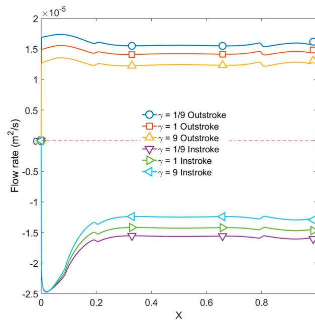
Figure 27. Flow rate per unit circumferential length at different asperity orientation in the instroke and outstroke motion. Piston velocity of 100 mm/s and sealed pressure of 10 MPa.
