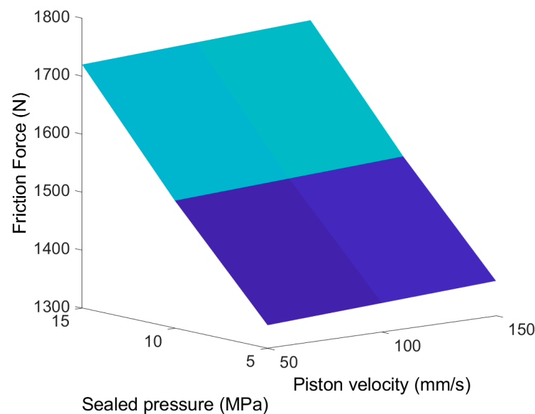
Figure 21. Variation in friction force with sealed pressure and piston velocity in the instroke direction with isotropic asperities ( \gamma = 1 ).
