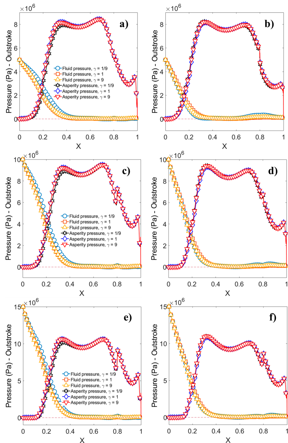
Figure 18. Fluid film and asperity contact pressure distribution with different sealing pressure and flow factors: (a,b) 5 MPa, (c,d) 10 MPa, (e,f) 15 MPa. Piston velocity: 100 mm/s.
