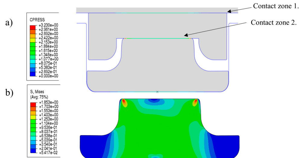
Figure 11. At the initial steps of the precompression stage, (a) contact pressure, (b) Von Mises stress distribution.
