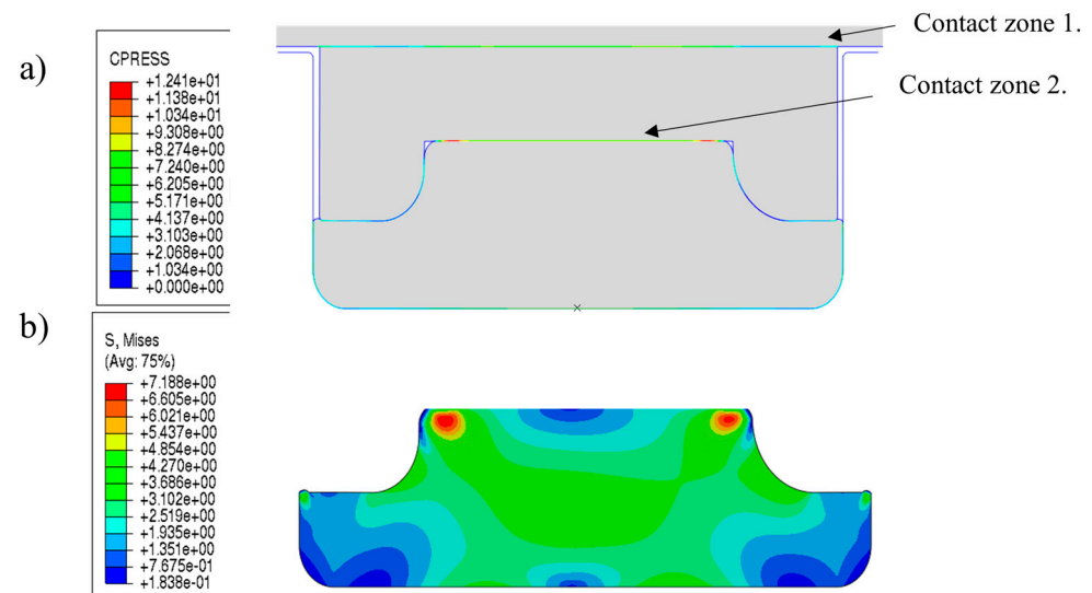
Figure 12. At full precompression, (a) contact pressure, (b) Von Mises stress distribution.
