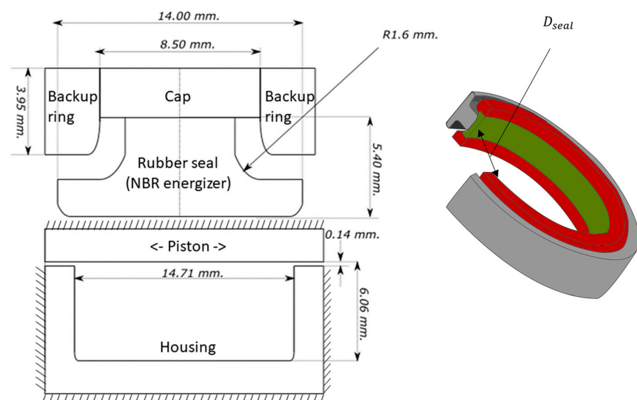
Figure 2. CTR seal and housing cross-sectional schematics, and CTR ring internal diameter.
