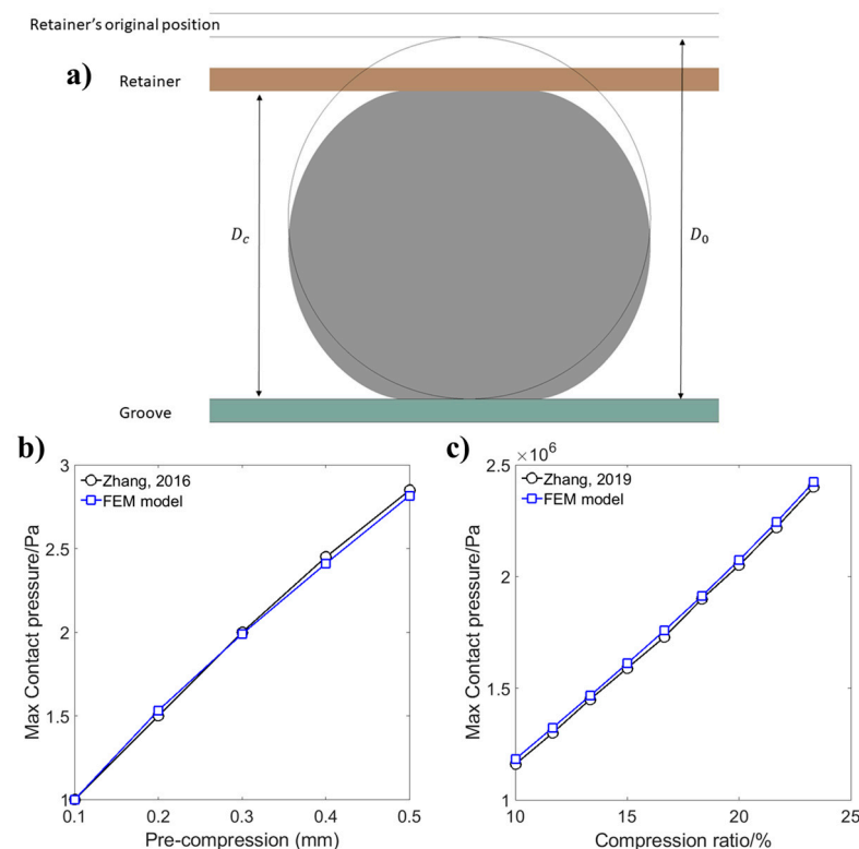
Figure 8. (a) Recreated O-ring model. (b) Maximum contact pressure at different pre-compressions. A comparison between Zhang et al. [10] and the present FEM model. (c) Maximum contact pressure at different compression ratios in comparison with Zhang et al. [7].
