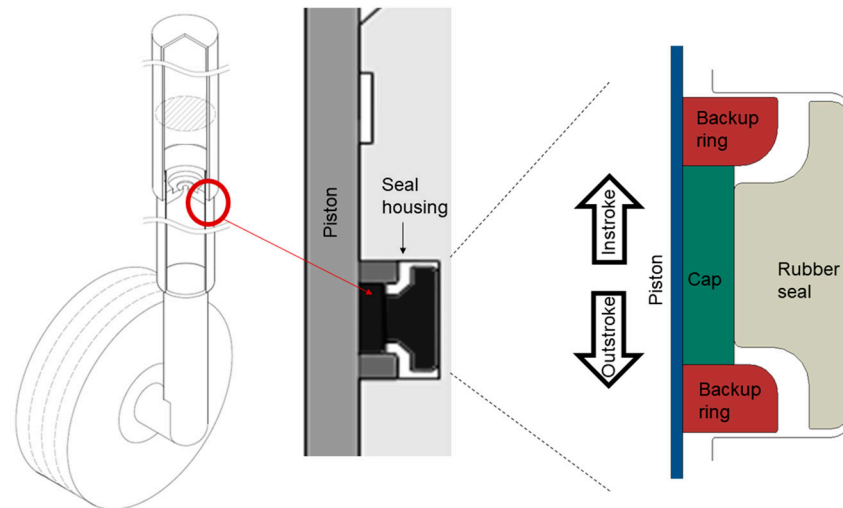
Figure 1. CTR seal and housing cross-sectional geometry, and schematic representation of the T-ring piston sealing system.
