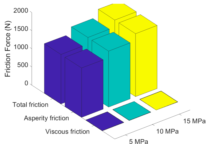
Figure 23. Friction force components at 5 MPa of sealed pressure and different piston velocities. Isotropic asperities.
