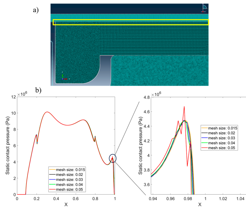
Figure 9. Mesh sensitivity analysis. (a) View of the mesh in the contact between the piston, a backup ring and the cap, denoted by yellow line, (b) contact pressure between the piston, backup rings and cap at different mesh sizes.
