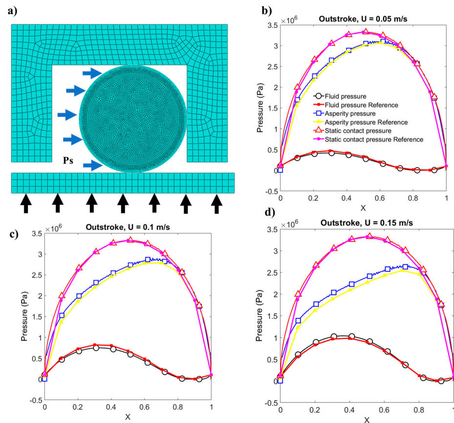
Figure 14. (a) Benchmark mesh and boundary conditions of verification case, recreated from [19]. Sealed pressure is 0.1 MPa, (b) pressure distributions in the outstroke direction with U = 0.05 m/s, (c) pressure distributions in the outstroke direction with U = 0.1 m/s, (d) pressure distributions in the outstroke direction with U = 0.15 m/s.
