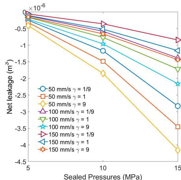
Figure 29. Net flow volume.
