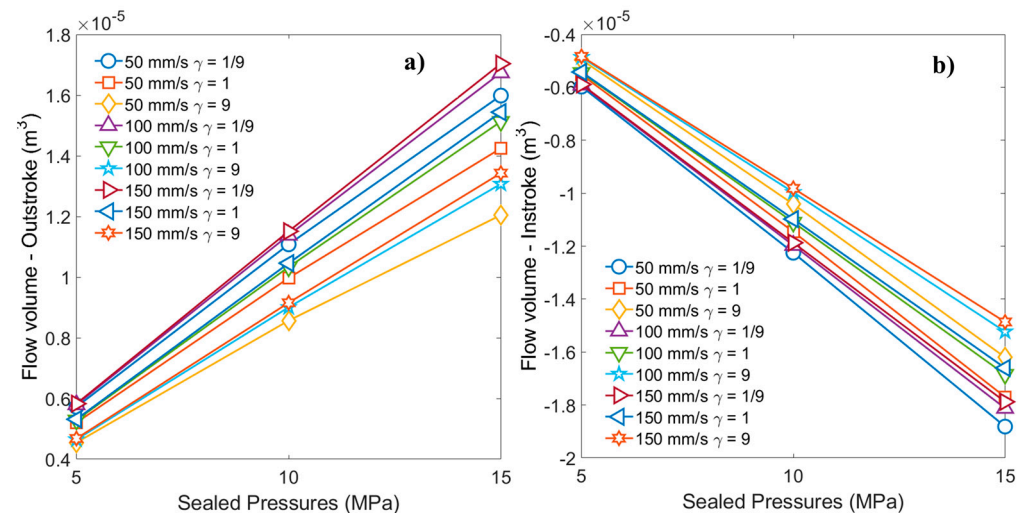
Figure 28. Flow volume in the (a) outstroke and (b) instroke motion.
