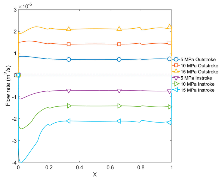
Figure 25. Flow rate per unit circumferential length at different sealed pressures in the instroke and outstroke motion. Isotropic asperities and piston velocity of 100 mm/s.
