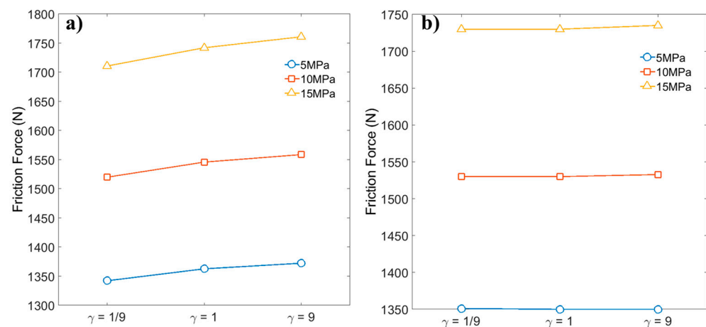
Figure 22. Friction force for different asperity orientations and sealed pressures. Piston velocity of 100 mm/s in the (a) outstroke and (b) instroke directions.
