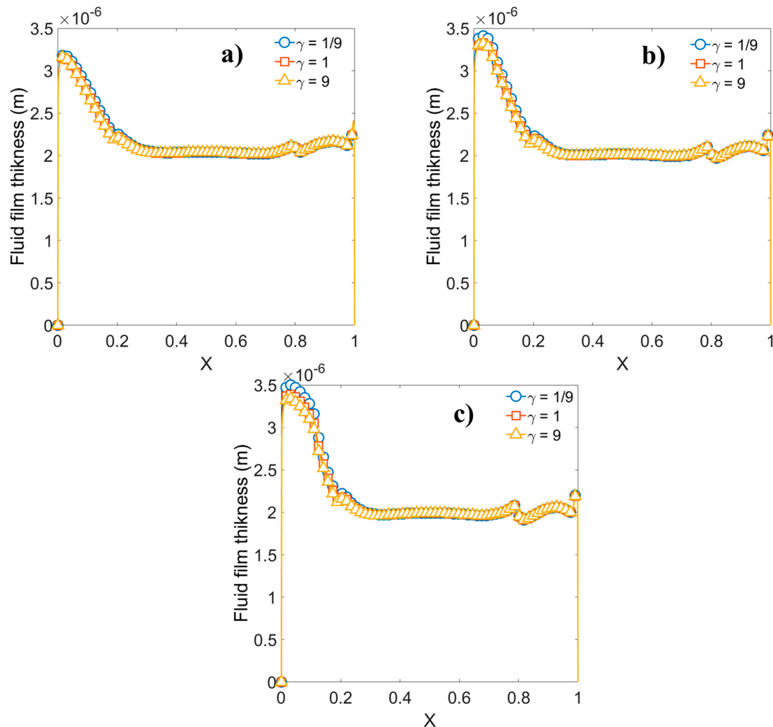
Figure 19. Fluid film thickness distribution for different \gamma values at 100 mm/s of piston velocity in the outstroke direction for: (a) 5 MPa sealed pressure, (b) 10 MPa sealed pressure, and (c) 15 MPa sealed pressure.
