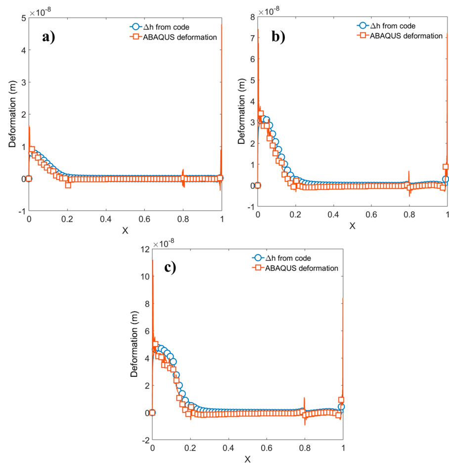
Figure 24. Elastic deformation comparison: (a) 5 MPa of sealed pressure, (b) 10 MPa of sealed pressure, (c) 15 MPa of sealed pressure.
