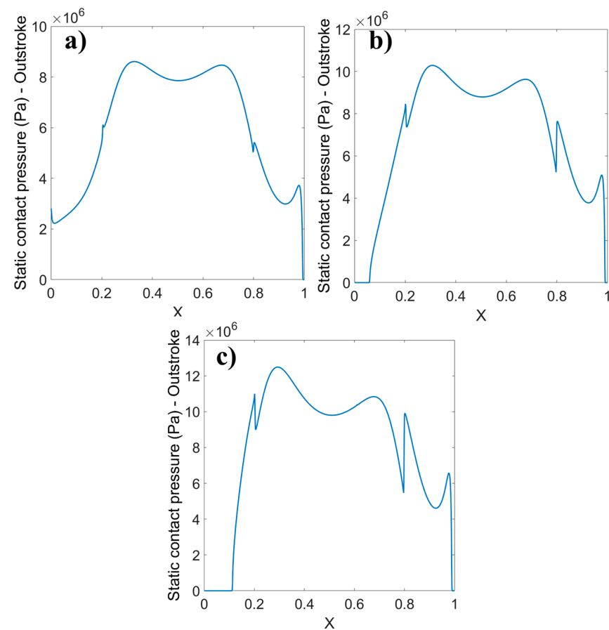
Figure 10. Static contact pressure distribution at sealed pressures of (a) 5 MPa, (b) 10 MP, (c) 15 MPa.
