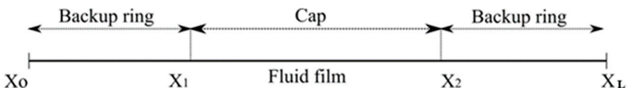
Figure 6. Fluid film channel discretized in 3 sections for different material parameters.
