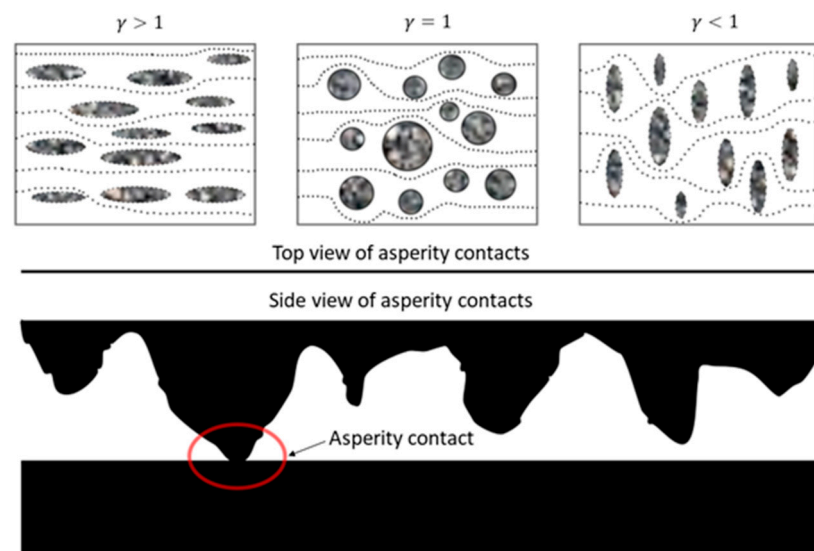
Figure 5. Top view of asperity contact orientations adapted from [27]. Side view of asperity contact between a rough and smooth surface.
