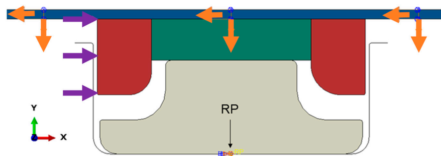
Figure 3. FEM model boundary condition. Orange arrows illustrate displacement boundaries, the precompression in the Y direction and the instroke–outstroke in the X direction. Magenta arrows represent the pressure boundary condition applied to the left part of the sealing assembly. RP stands for reference point in the groove.
