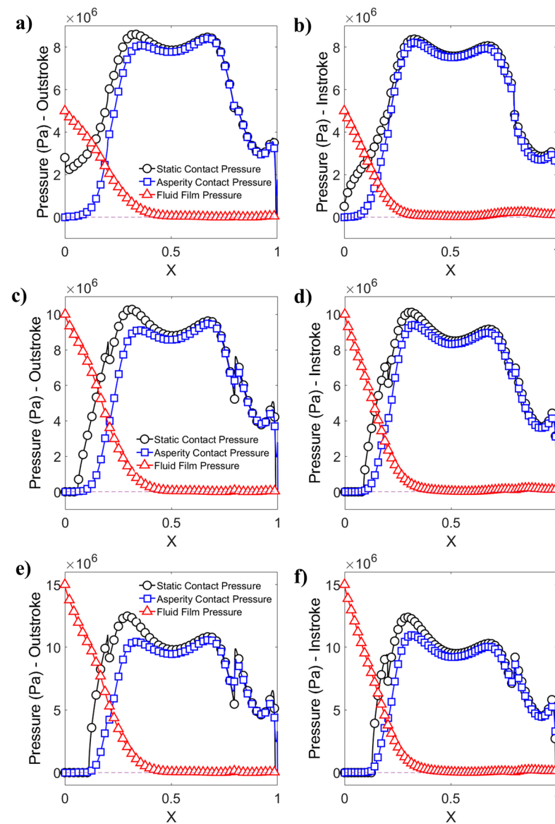
Figure 15. Pressure distributions at different sealed pressures in the instroke and outstroke directions: (a,b) 5 MPa, (c,d) 10 MPa, (e,f) 15 MPa.
