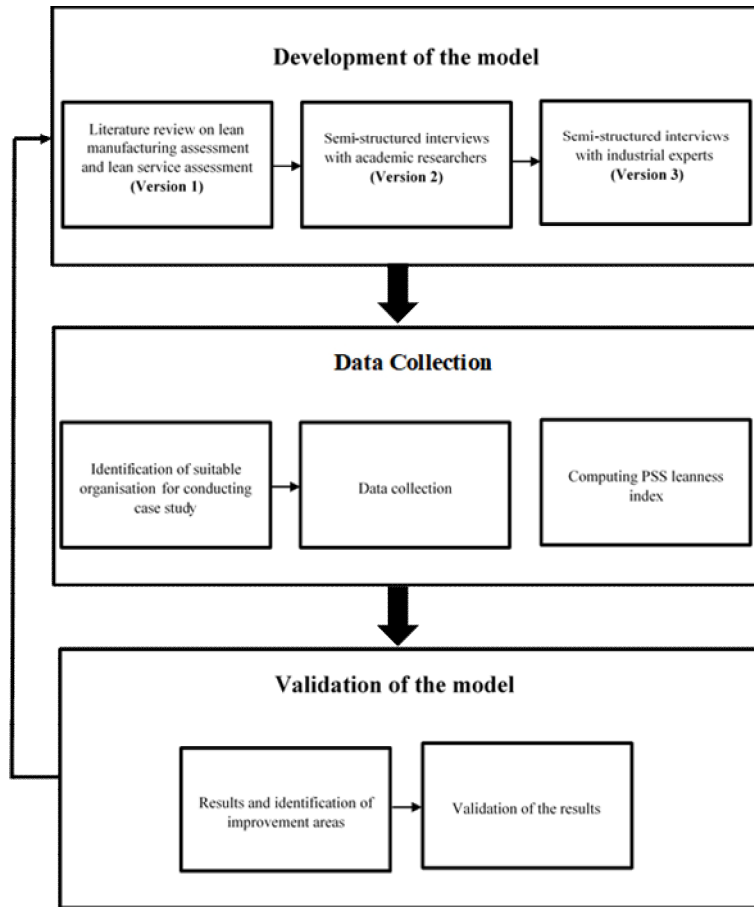
Figure 1. Research methodology
