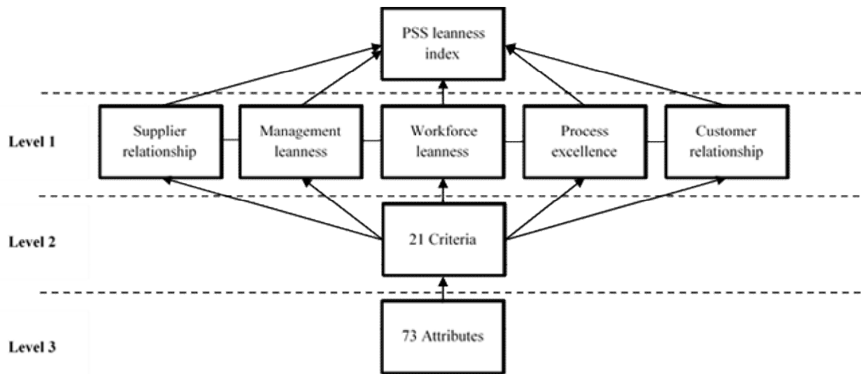
Figure 2. Assessment model
