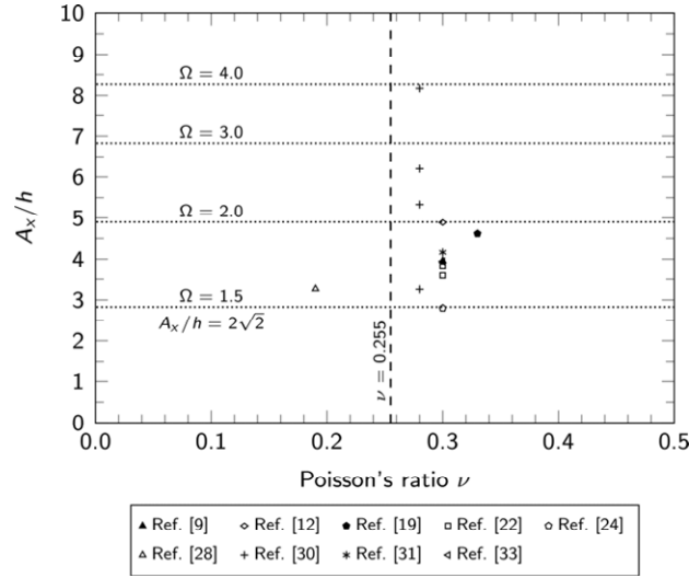
Fig. 4. Validation of the condition of TCB formation, namely, that \Omega > 3/2 from Eq. (3), or equivalently, that A_x/h > 2\sqrt{2} from Eq. (11).
