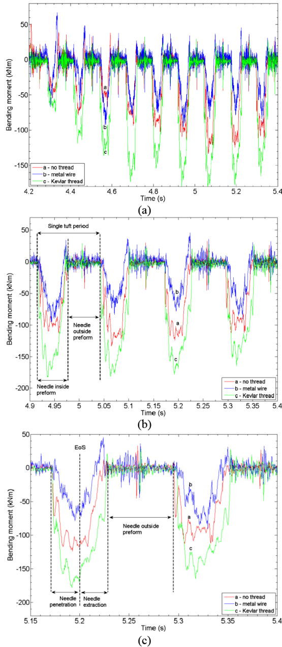
Figure 9. Bending moment in the left–right plane of the needle evaluated from the signals measured by 4 FBG sensors showing (a) several tuft periods, (b) \sim 3 tuft periods and (c) \sim 1 tuft period. A 4 layer quasi-isotropic preform was tufted at a speed of 500 rpm by a needle without thread, with metal wire and Kevlar ® thread. EoS: end of stroke.
