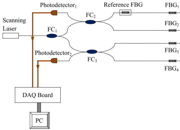
Figure 3. Schematic diagram of the experimental lay-out showing the FBG sensor interrogation system. FC1–FC3: fibre optic directional couplers (50/50 split ratio), FBG1–FBG4: FBGs surfaced-bonded to the needle, DAQ: data acquisition board, PC: personal computer.
