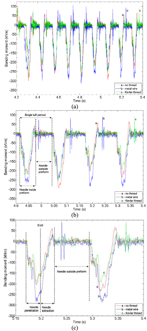
Figure 10. Bending moment in the back–front plane of the needle evaluated from the signals measured by 4 FBG sensors showing (a) several tuft periods, (b) \sim 3 tuft periods and (c) \sim 1 tuft period. A 4 layer quasi-isotropic preform was tufted at a speed of 500 rpm by a needle without thread, with metal wire and Kevlar ® thread. EoS: end of stroke.
