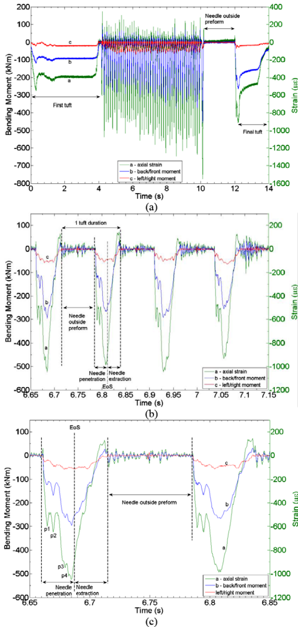
Figure 7. Axial strain and bending moments evaluated from 4 FBG signals of figure 5: (a) an entire tuft process over the whole length of preform, (b) \sim 3 tuft periods and (c) \sim 1 tuft period. A 4 layer quasi-isotropic preform was tufted by a thread-less needle at a tufting speed of 500 rpm. p1–p4: troughs, EoS: end of stroke.
