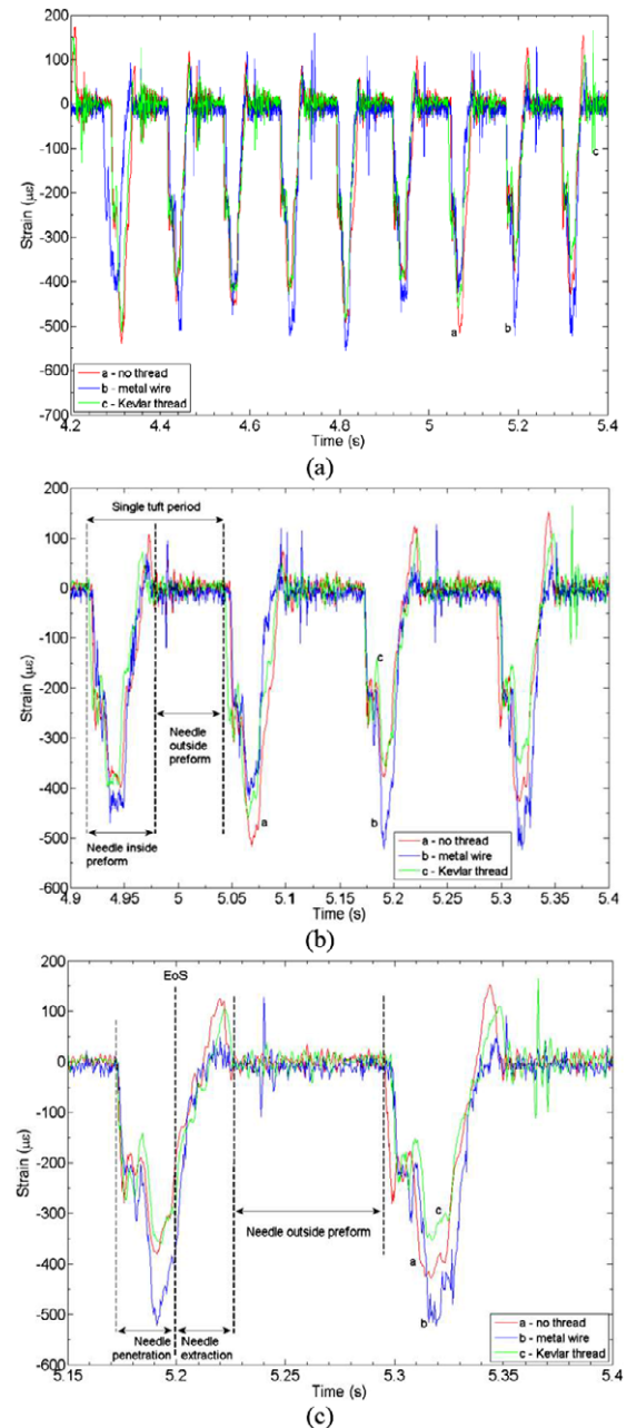
Figure 8. Axial strain in the needle evaluated from the signals measured by 4 FBG sensors showing (a) several tuft periods, (b) \sim 3 tuft periods and (c) \sim 1 tuft period. A 4 layer quasi-isotropic preform was tufted at a speed of 500 rpm by a needle without thread, with metal wire and Kevlar ® thread. EoS: end of stroke.
