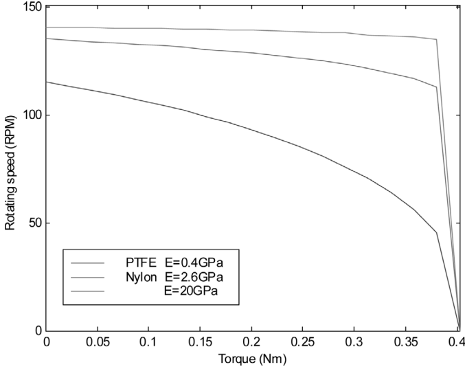
Fig. 5. Motor speed against external loads applied for different contact layer material where P = -80 N, V = 150 V, \omega = 1.0355\omega_n , h_c = 0.5 mm, \mu = 0.18 , and \zeta = 1\% .
