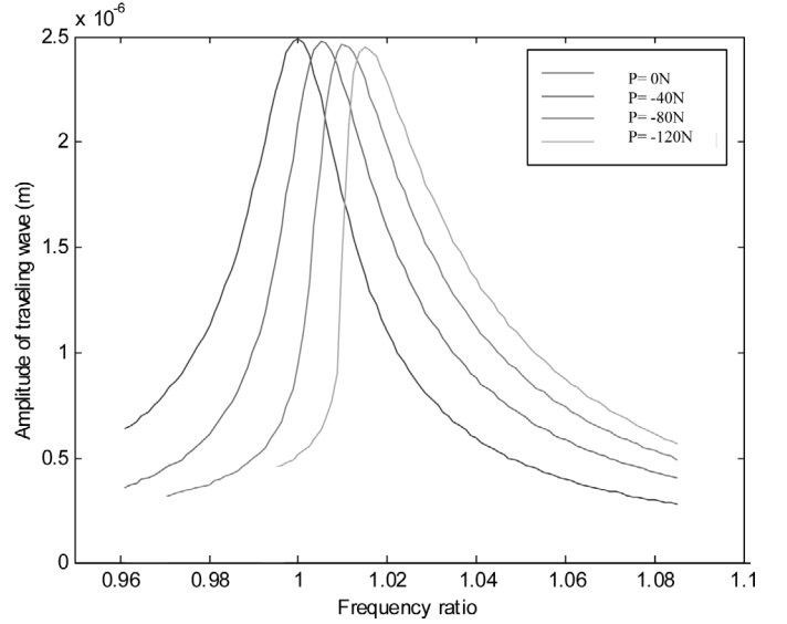
Fig. 7. Frequency response of the amplitude of the traveling wave of the stator for different compressive forces in which the material contact layer is PTFE, E = 0.4 GPa, M_{\text{applied}} = 0.15 Nm, V = 150 V, h_c = 0.5 mm, \mu = 0.18 , and \zeta = 1\% .
