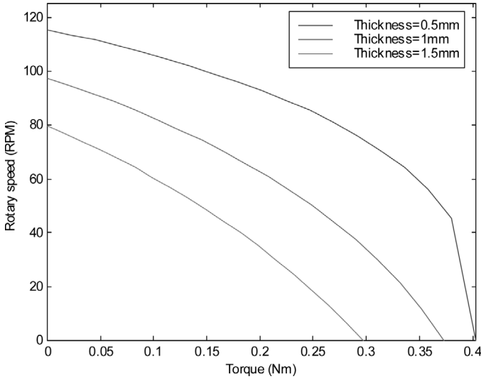
Fig. 6. Load response of rotation speed of the rotor for different thickness of the contact layer where the contact-layer material is PTFE, P = 80 N, V = 150 V, \omega = 1.0355\omega_n , h_c = 0.5 mm, \mu = 0.18 , and \zeta = 1\% .
