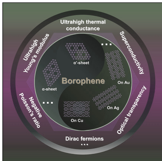
Fig. .12. Various borophene structures and their unique physical properties, including mechanical compliance, anisotropic electronic structure, optical transparency, high thermal conductance, and phonon-mediated superconductivity [158].
