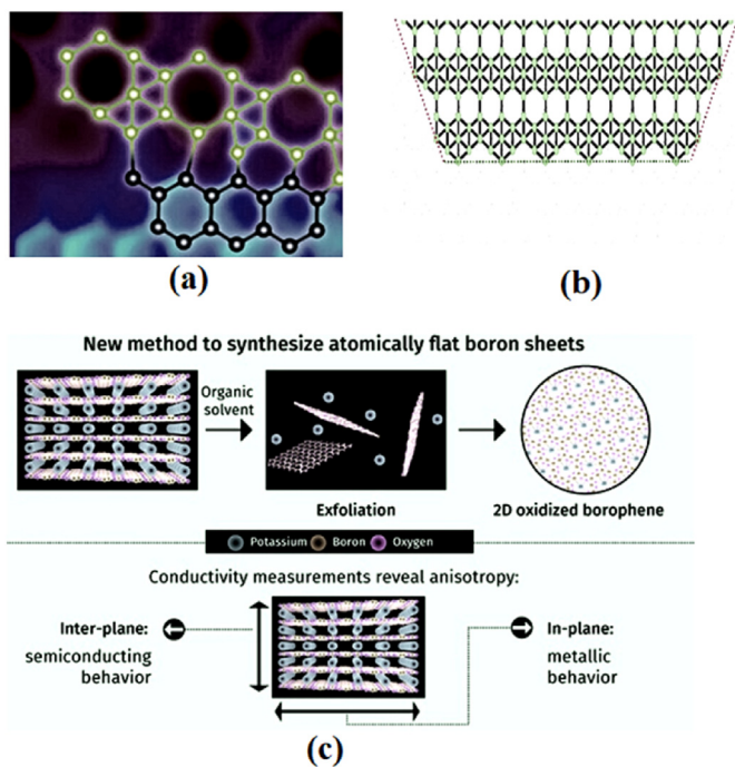
Fig. 8. (a) Atomic-resolution scanning tunnelling microscopy image of a borophene-graphene lateral heterostructure with an overlaid schematic of interfacial boron-carbon bonding [143], (b) Edges connected at the corners of a borophene flake [144], (c) The bottom-up synthesis of crystalline-stacked boron atomic layers from a solution process, conductivity measurements revealed the electronic feature, activation energy of the in-plane conductivity suggested a metal-like behaviour whereas that of the interplane showed a semiconducting nature [111].
