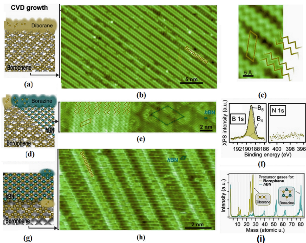
Fig. 7. (a) CVD growth of borophene and borophene-hBN heterostructures on Ir(111) is shown in schematic with diborane dosage, (b) STM image of single-crystalline borophene on Ir(111), and (c) details its structure, (d) Sequential borazine and diborane dosage create borophene-hBN lateral heterostructures, (e) High-res STM image of borophene's wavy appearance and hBN's hexagonal moiré pattern, (f) XPS spectra confirm boron and nitrogen 1s core levels, (g) Vertical heterostructure formation, (h) atomically resolved hBN lattice, (i) Mass spectra of diborane and borazine gases [6].
