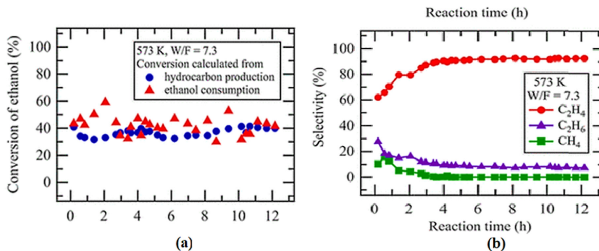
Fig. 14. (a) Conversion of ethanol on hydrogenated borophene (HB) sheets as a function of reaction time at 573 K and W/F = 7.3 g min/mmole, estimated from hydrocarbon production (blue circles) and ethanol consumption (red triangles). (b) Selectivity vs reaction time [267].
