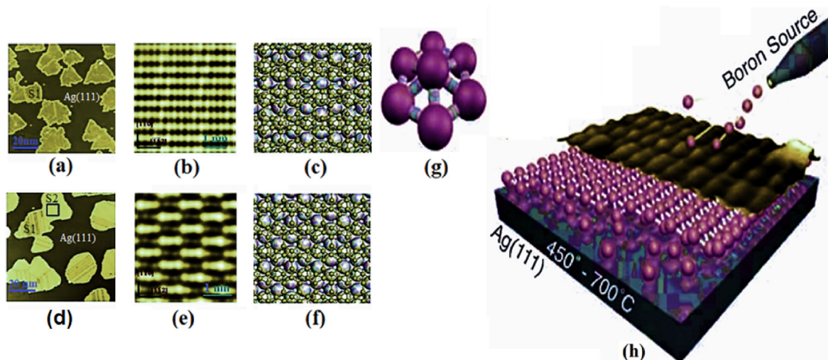
Fig. 3. (a, d) Large-scale scanning tunnelling microscopy (STM) images provide an overview of monolayer borophene islands on the Ag (111) substrate, (b, e) High-resolution STM images reveal finer details within these borophene islands, (c, f) Atomic structure models depict triangular boron lattices with periodic boron vacancy arrangements of borophene on the silver substrate [106], (g-h) Synthesis of borophenes: Anisotropic, two-dimensional boron polymorphs [90].
