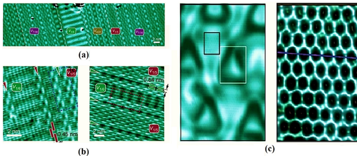
Fig. 9. (a) Atomic-resolution scanning tunnelling microscopy image of a borophene-graphene lateral heterostructure with an overlaid schematic of interfacial boron-carbon bonding [143], (b) Edges connected at the corners of a borophene flake [144], (c) Bottom-up synthesis of crystalline-stacked boron layers from a solution process revealed metal-like in-plane conductivity and semiconducting interplane conductivity [111], high-resolution STM images displayed a borophene monolayer with a honeycomb lattice on Al (1 1 1) [147].
