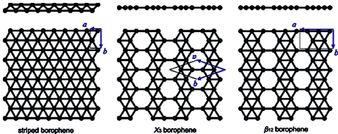
Fig. 13. Crystal structures of experimentally obtained borophenes: Striped borophene (a non-flat borophene form), \beta_{12} borophene (a.k.a. \gamma sheet or \sqrt{1/6} sheet), \chi_3 borophene (a.k.a. \sqrt{1/5} sheet) [168].
