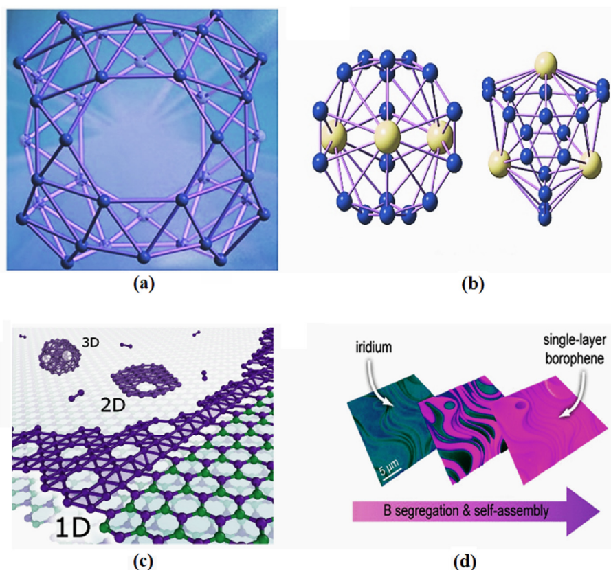
Fig. 6. (a) Clusters of 40 boron atoms form a molecular cage similar to the carbon buckyball. This is the first experimental evidence that such a boron cage structure exists [128], (b) The family of boron-based nanostructures has a new member: metallo-borospherene, hollow cages made from 18 boron atoms and three atoms of lanthanide elements [136], (c) Borophene Growth on Hexagonal Boron Nitride: Enabling Easy Separation, Reduced Nucleation Dimensionality, and Lowered Barriers for Enhanced Property Evaluation [105], (d) Segregation-Enhanced Epitaxy of Borophene on Ir(111) by Thermal Decomposition of Borazine [137].
