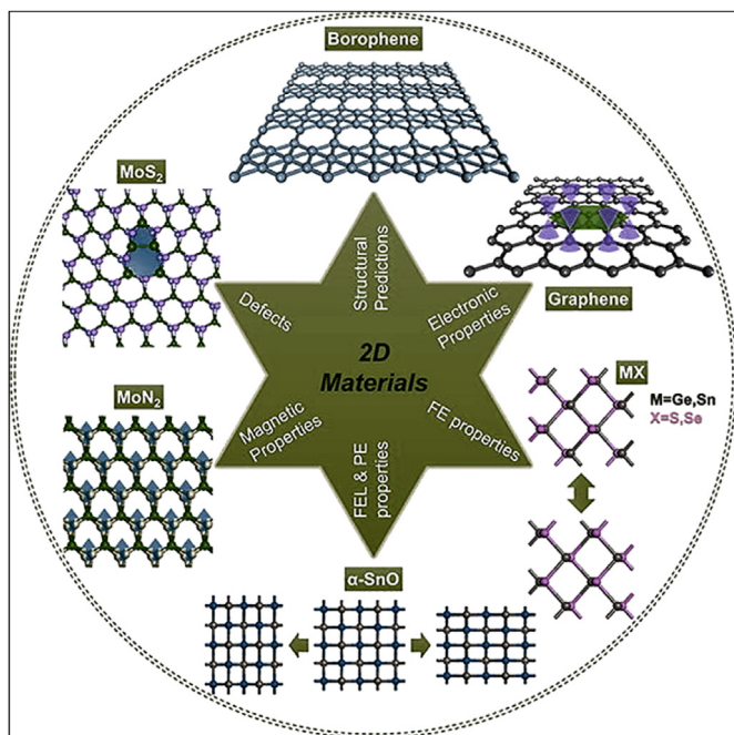
Fig. .11. Structure and Properties of Two-Dimensional Nanostructures" in the context of Design and Property Predictions [153].
