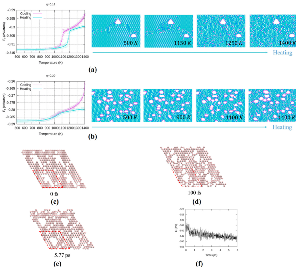
Fig. 10. Energy and configuration changes during heating for (a) \eta = 0.14 , and (b) \eta = 0.2 , Ab initio molecular dynamics for a 10 \times 10 borophene supercell during cooling from 2400 K to 1800 K with 0.1 \text{ K fs}^{-1} cooling rate. (c)–(e) Borophene configurations at specific times: (c) initial, (d) 100 fs, and (e) 5.77 ps and (f) the potential energy during the cooling (the red dashed lines denote the unit cell used in the simulations) [145].
