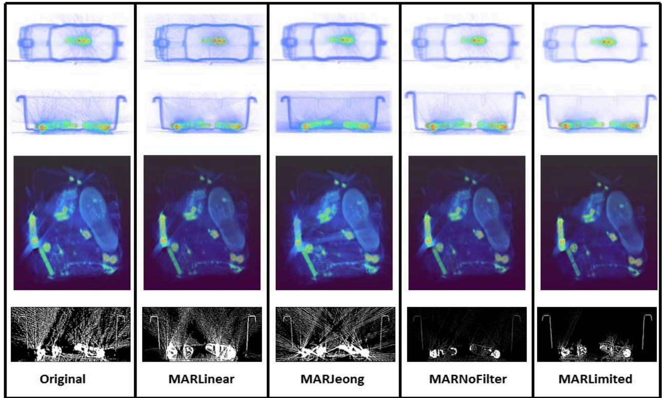
Fig. 2. Visual comparison results.
