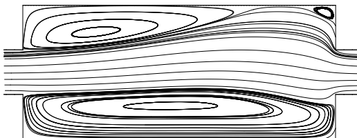
Figure 3: Re=120 HLLE scheme in conjunction with third-order interpolation accuracy.
