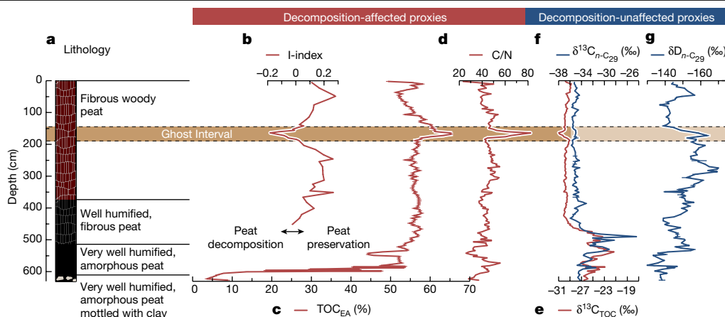
Fig. 2 | Stratigraphy, decomposition-affected and decomposition-unaffected geochemical properties for peat core CEN-17.4. a , Lithology. b , I-index (I for immature), indicating the preservation of thermally labile immature organic matter 9 . Note that I-index values of fresh organic matter ranges from 0.2 to 0.5 (ref. 9 ). c , Total organic carbon (TOC EA ). d , Carbon-to-nitrogen ratio (C/N). e , Carbon isotopes of total organic carbon (TOC) (δ 13 C TOC ). f , Carbon isotopes of n -C 29 alkanes from plant waxes (δ 13 C n -C 29 ). g , Hydrogen isotopes of n -C 29 alkanes from plant waxes (δD n -C 29 ). Proxy indicators are classified as decomposition-
