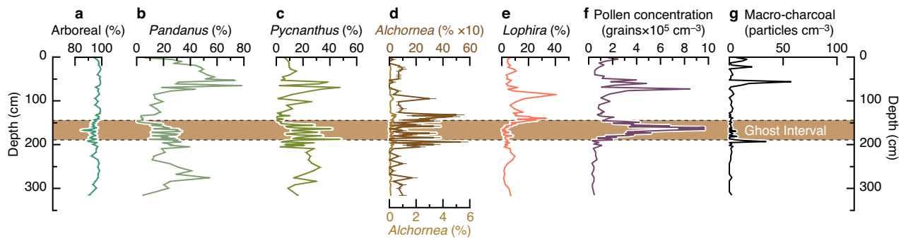
Extended Data Fig. 4 | Core CEN-17.4 pollen and macro-charcoal data.
