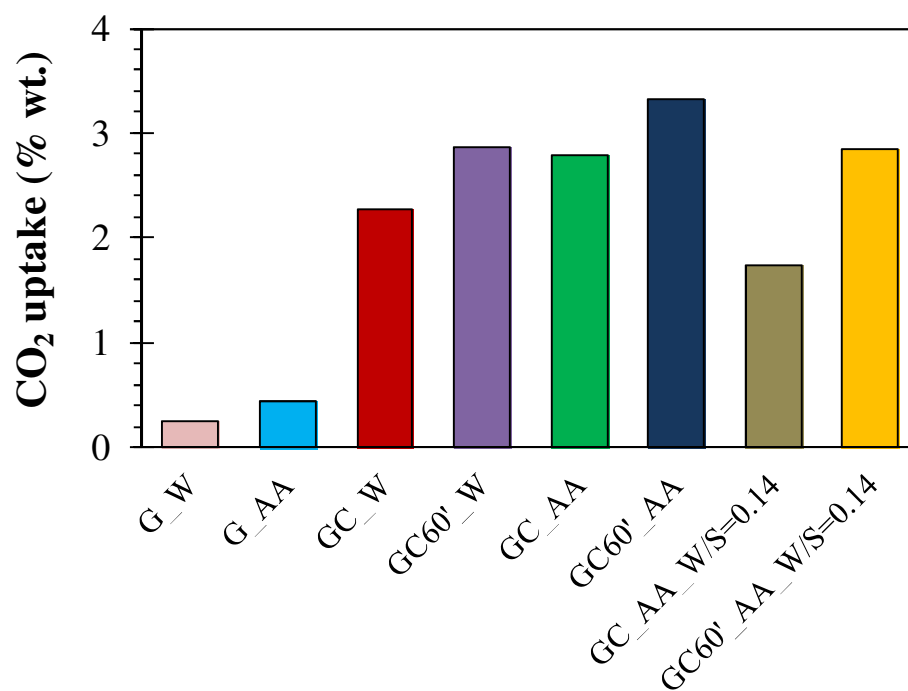
Figure 2. CO 2 uptake of the granules obtained after the tested treatments (see Table 2 for the explanation of the experiment codes reported on the x-axis).
