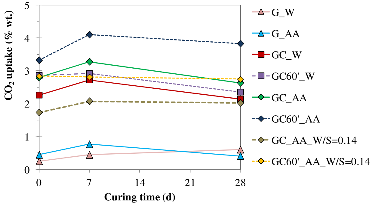
Figure 3. CO 2 uptake with curing time of the granules obtained applying the different types of treatments tested (see Table 2 for the explanation of the experiment codes reported in the legend).
