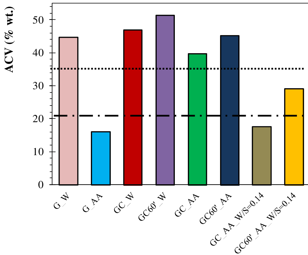
Figure 5. ACV of the granules obtained from the different treatments tested compared to the values reported for mixed gravel (21%) and blast furnace slag (35%) (British Standard, 1990), see Table 2 for the explanation of the experiment codes reported on the x-axis.
