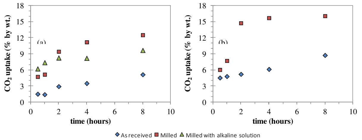
Figure 4. CO 2 uptake kinetics of BOF slag resulting from the batch tests: a) at ambient conditions (T=20 °C, p=1 bar, L/S=0.3 l/kg) and b) at enhanced conditions (T=50 °C, p=10 bar, L/S=0.3 l/kg).
