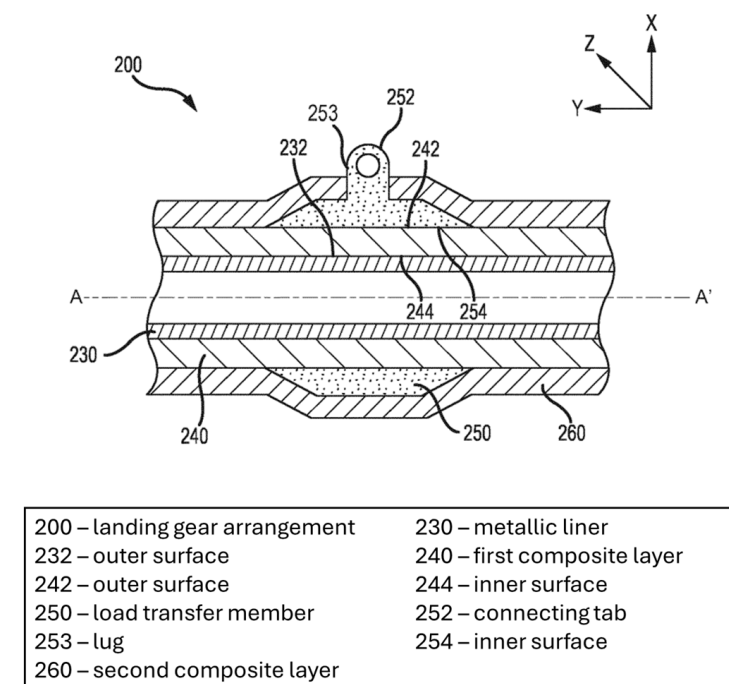
Figure 2. An axial cross-section view of a landing gear arrangement, in accordance with various embodiments [26].
