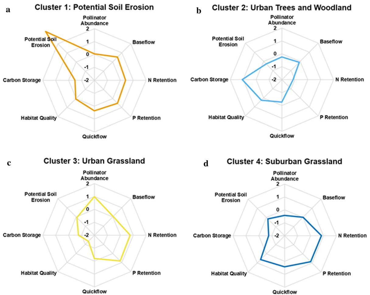
Fig. 3 Radar charts showing Ecosystem Service Bundle types and the provision of different ES in a cluster. K-means cluster analysis revealed four distinct ecosystem service bundle types. The charts show the average values of each service in the bundle type. a Cluster 1: Potential Soil Erosion bundle type, b Cluster
